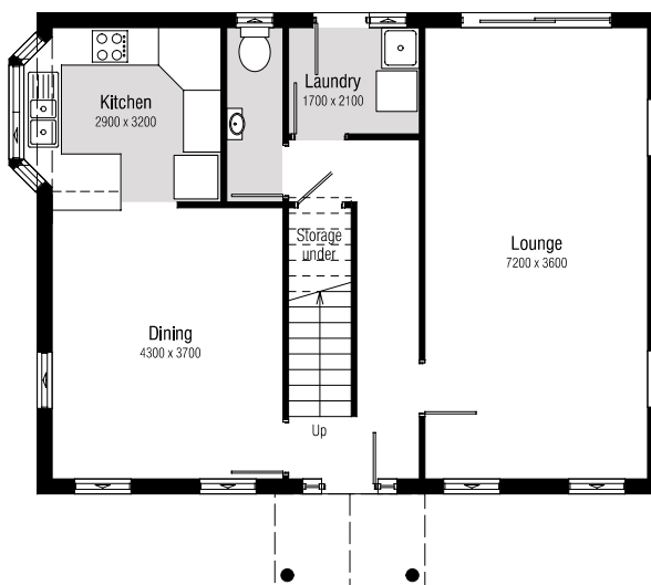
LOWER FLOOR LAYOUT
