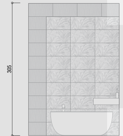
Wall B
