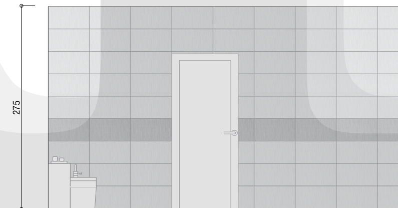
Wall D
