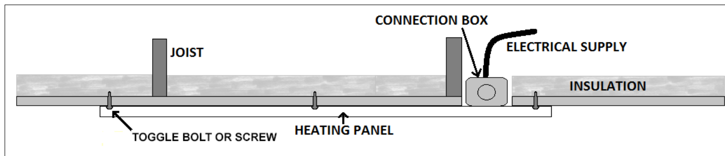
Figure 1 – Surface Mounting
