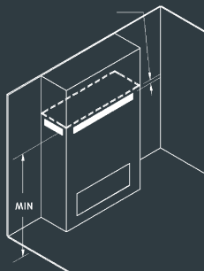
Framing to ceiling, minimum enclosure with front or side vents
