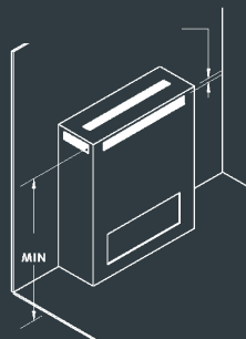
Minimum enclosure with front or side vents
