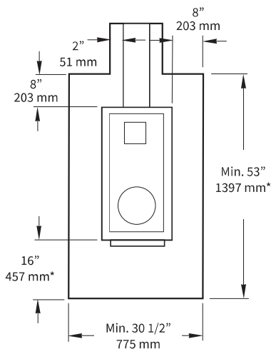
Figure 19. Minimum Hearth Dimensions.
