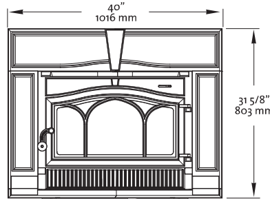
Figure 73. Dimensioned Views
