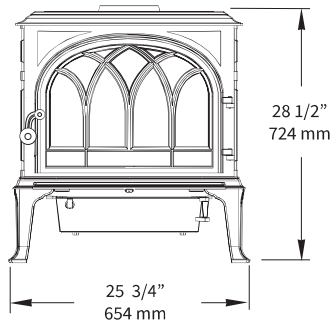
Figure 39. F 400 Castine dimensions. See clearance chart for flue collar centerline positions.
