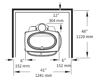
Figure 54 Alcove w/ wall protection.
