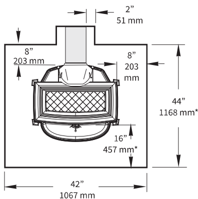
Figure 38. Minimum Hearth Dimensions.
