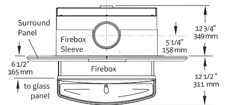
Figure 66. Minimum Sleeve Adjustment.
