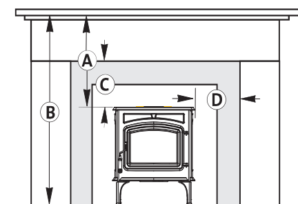
Figure 63. Alcove with wall protection.
