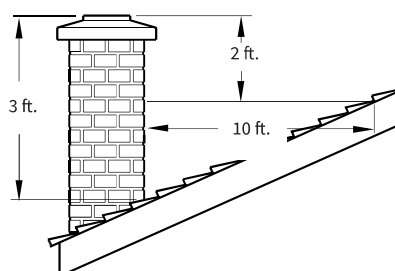
Figure 1. The 3' / 2' / 10' Chimney Rule.
