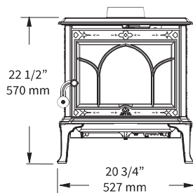
Figure 27. F 100 Nordic QT overall dimensions. See clearance chart for flue collar centerline positions.
