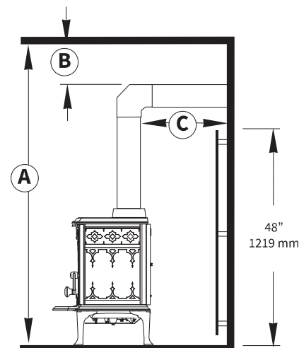
Figure 31. Alcove with Wall Protection
