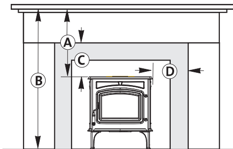
Figure 63. Alcove with wall protection.
