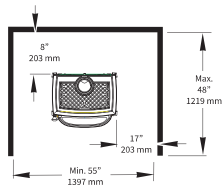
Figure 29. Alcove without Wall Protection
