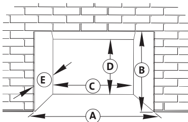
Figure 62. Minimum Fireplace Requirements
