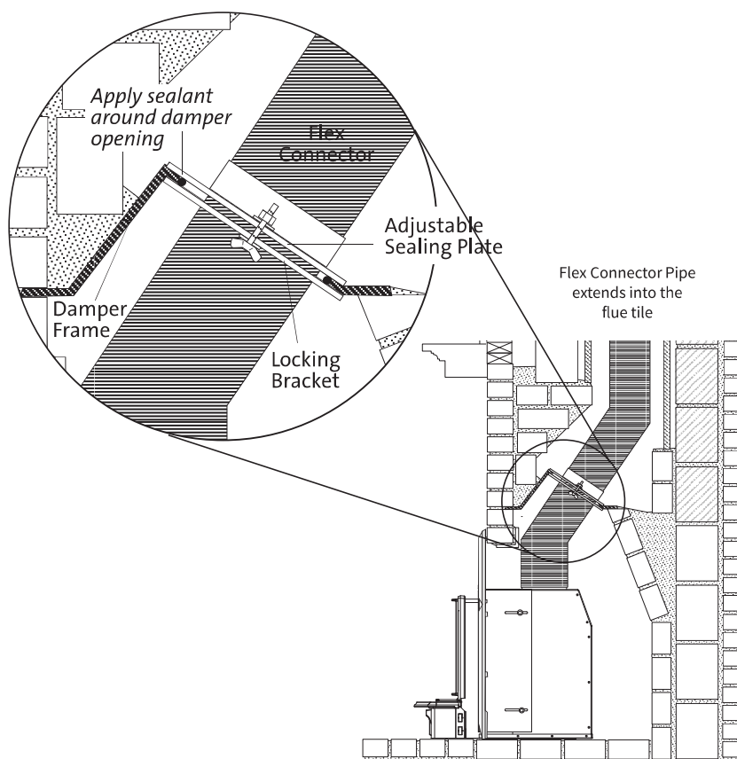
Figure 78. Positive Chimney Connection - U.S.
