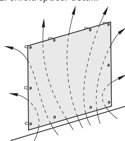
Figure 12. Open wall shield construction. Do not install spacers directly behind the stove or connector.
