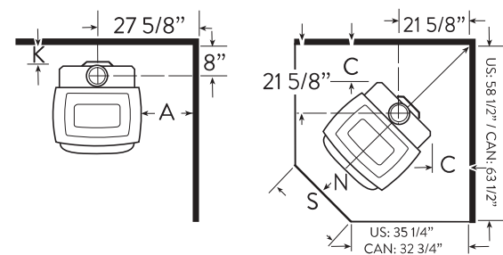
Double Wall Connector with Flue Collar Heat Shield
