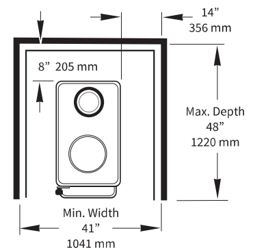
Figure 17. Alcove stove clearance with Double-wall pipe and wall protection.
