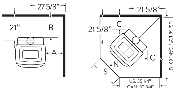
Single Wall Connector
