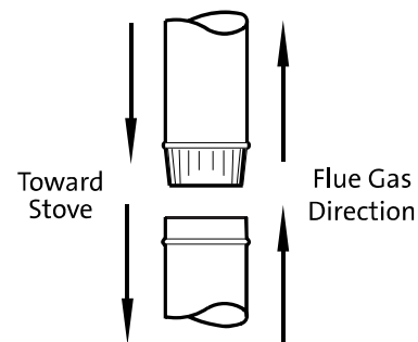
Figure 2. Assemble chimney connection sections crimped end toward stove.
