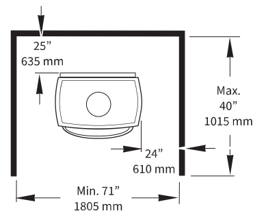
Figure 35. Alcove with no Wall Protection
