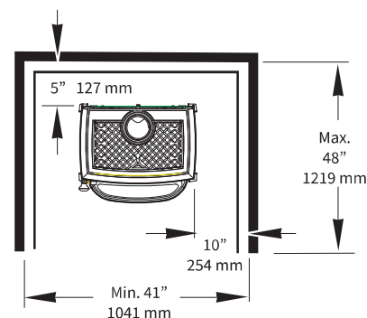
Figure 30. Alcove with Wall Protection
