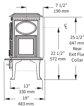
Figure 33. F 3 CB overall dimensions. See clearance chart for flue collar centerline positions.
