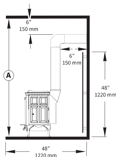
Figure 55. Alcove Ceiling and Double-wall Connector Clearances.
