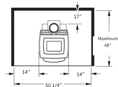
Figure 62. Alcove with no wall protection.
