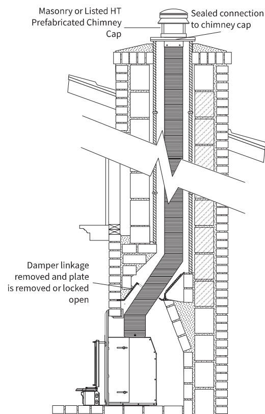
Figure 79. Positive Chimney Connection - Canada.
