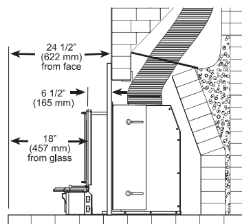
Figure 71. Provide hearth protection to accommodate maximum firebox extension forward of fireplace face.
