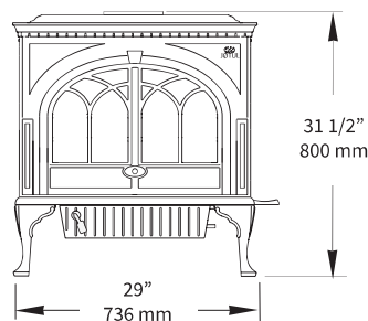
Figure 51. F 600 Firelight CB dimensions. See clearance chart for flue collar centerline positions.
