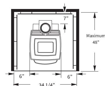
Figure 63. Alcove with wall protection.
