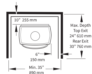
Figure 36. Alcove with Wall Protection
