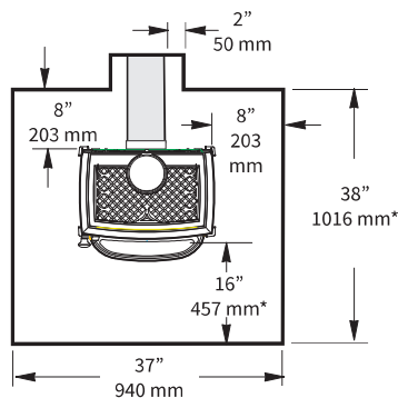
Figure 26. Minimum Hearth Dimensions. * Denotes requirement for Canada.
