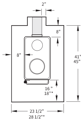
Figure 13. Minimum Hearth Dimensions. * Denotes requirement for Canada.
