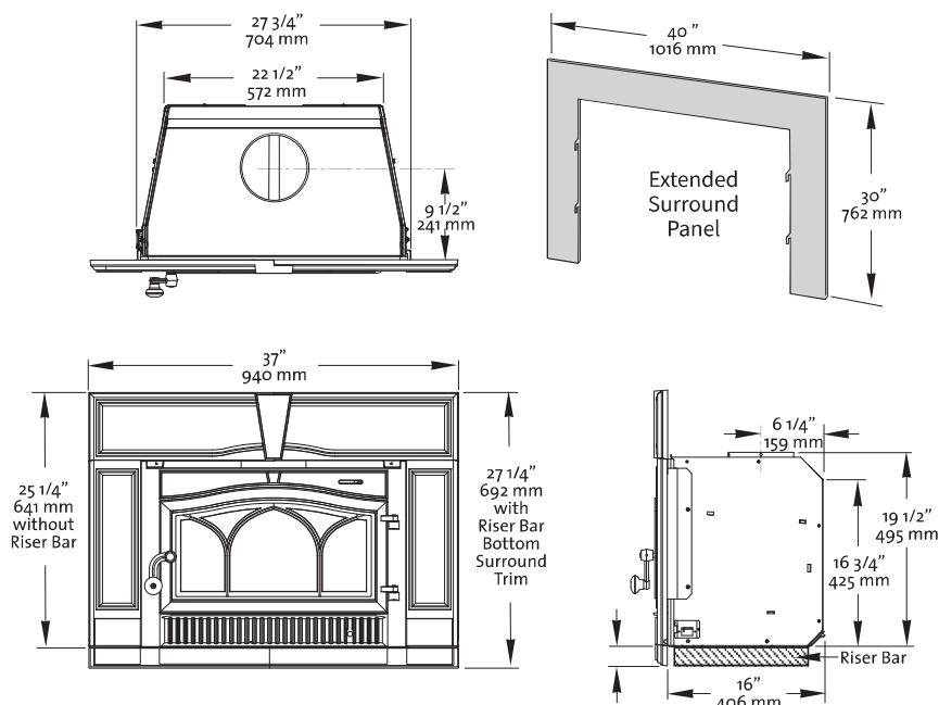
Figure 57. Dimensioned Views
