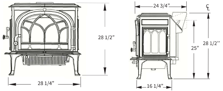
Figure 48. F 500 Oslo dimensions. See clearance chart for flue collar centerline positions.
