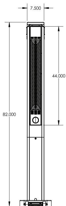
FRONT VIEW
