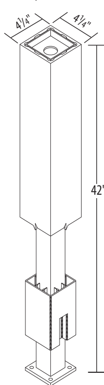
Newel-Loc™ Square Newel Post Mount Sleeve Support
