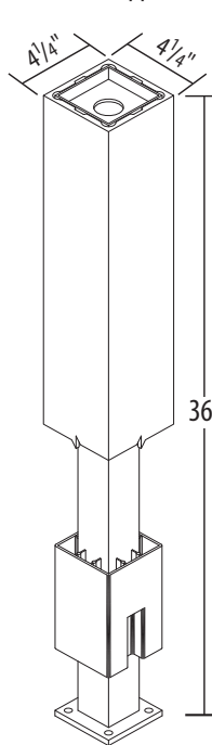
Newel-Loc™ Square Newel Post Mount Sleeve Support
