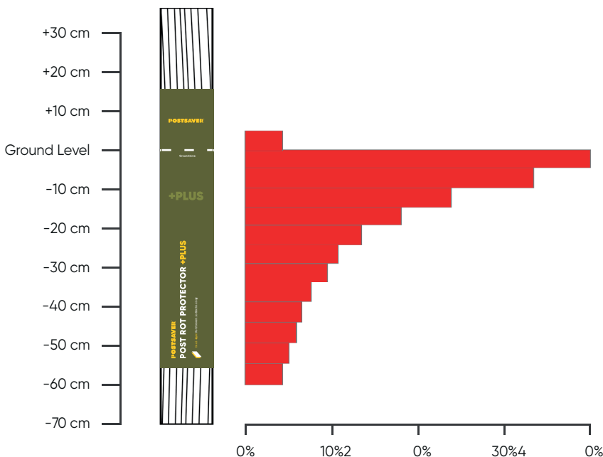
Graph showing Typical likelihood/rate of decay vs depth below ground level
