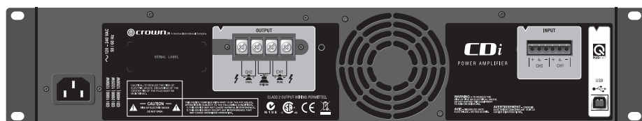
CDi 1000, 2000, 4000 back panel
