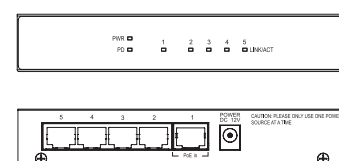
SE-5-EP 5-Port Unmanaged Switch, PoE Powered 5.86 × 3.30 × 1.02" (149 × 84 × 26 mm)
