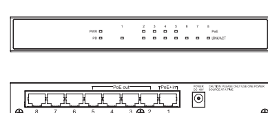
SE-8P2-EPA 8-Port Unmanaged Switch, PoE+ or AC Powered, 4 PoE Out 7.59 × 3.30 × 1.02" (142 × 90 × 22 mm)
