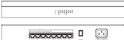
SE-8P 8-Port Unmanaged Switch with 8 PoE or Up to 4 PoE+ 12.68 × 7.30 × 1.73" (142 × 90 × 22 mm)
