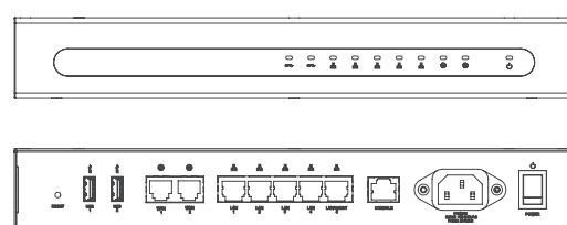
RK-1 7-Port Gigabit Router 12 × 7.5 × 1.75" (305 × 190 × 44 mm)
