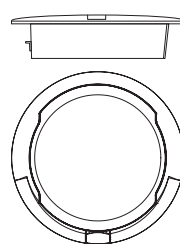
WK-1-C 802.11ac 2x2 Access Point, In-Ceiling 10.29 x 3" – radius 4.5" (261 x 76 mm – radius 114 mm)
