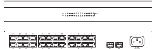
SE-26 26-Port Unmanaged Switch with 2 Fiber 12.68 × 7.30 × 1.73" (322 × 185 × 44 mm)
