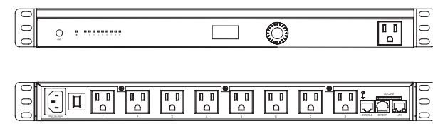
PE-09N PowerPak 9-Outlet Intelligent Power Distribution Unit, Surge Protected 17.15 × 11.48 × 1.75" (434 × 292 × 45 mm)
