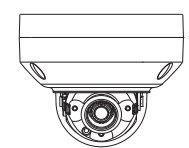
CK-CAM-IN302 Indoor Dome Camera 4.33 × 4.33 × 3.50" (110 × 110 × 89 mm)
