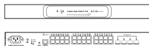
S3L-24P 24-Port Layer 3 Lite Managed Switch with 24 PoE or Up to 12 PoE+, 4 SFP+ 17.32 × 8.27 × 1.73" (440 × 210 × 44 mm)
