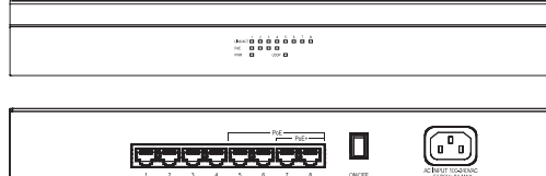
SE-8P4 8-Port Unmanaged Switch with 4 PoE or Up to 2 PoE+ 12.68 × 7.30 × 1.73" (322 × 185 × 44 mm)
