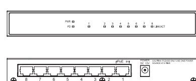
SE-8-EP 8-Port Unmanaged Switch, PoE Powered 7.59 × 3.30 × 1.02" (193 × 84 × 26 mm)
