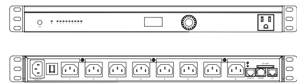
PE-08I PowerPak 8-Outlet Intelligent Power Distribution Unit, Surge Protected, International 17.15 × 11.48 × 1.75" (434 × 292 × 45 mm)
