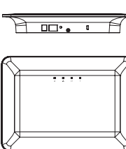
WX-1 802.11ac 3x3 Access Point, Plenum Rated 9.80 × 7.05 × 1.43" (249 × 179 × 36 mm)
