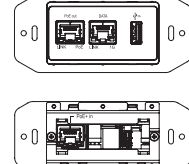
SE-USB1-EP 3-Port Unmanaged Switch with USB, 1 PoE+ Powered, 1 PoE Out, 1 Data Out 4.25 × 1.9 × 2.4" (108 × 48 × 61 mm)
