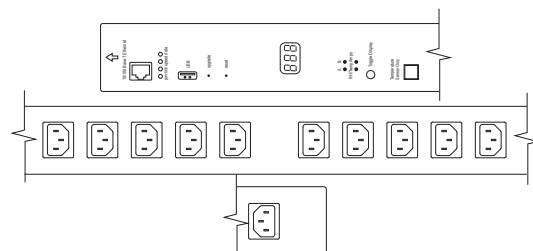
P20E 20-Outlet Intelligent Power Distribution Unit, International 55.00 × 2.75 × 2.00" (1,397 × 70 × 51 mm)
