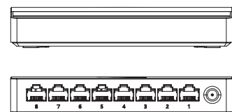
SE-8 8-Port Unmanaged Switch, Desktop 5.59 × 3.54 × 0.87" (142 × 90 × 22 mm)
