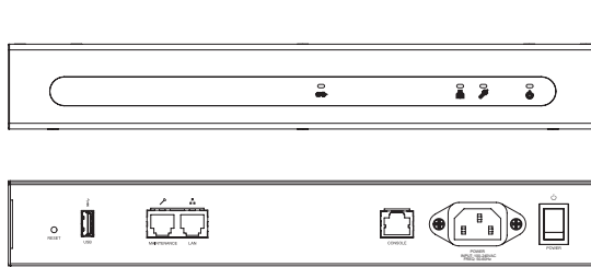
NK1-CP1 Wireless Controller for up to 15 Access Points 12.00 × 7.50 × 1.75" (305 × 191 × 45 mm)
