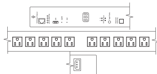
P20 20-Outlet Intelligent Power Distribution Unit 55.00 × 2.75 × 2.00" (1,397 × 70 × 51 mm)
