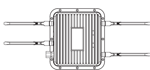
WK-1-O 802.11ac 2x2 Access Point, Outdoor 10.59 x 9.41 x 3.26" (269 x 239 x 83 mm)
