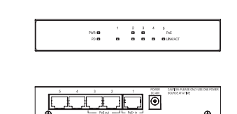
SE-5P2-EPA 5-Port Unmanaged Switch, PoE+ or AC Powered, 2 PoE Out 5.86 × 3.30 × 1.02" (108 × 48 × 61 mm)
