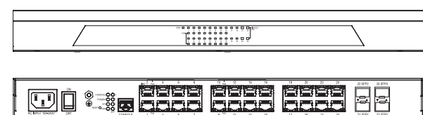
SX-24P16 24-Port Managed Switch with 16 PoE or Up to 8 PoE+ 17.13 × 12.21 × 1.75" (435 × 310 × 44 mm)
