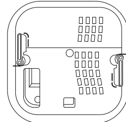
ICBKT-WA-2200 WA-2200 In-Ceiling Mounting Bracket 8.72 x 8.72 x 3.44" (222 x 221 x 87.4 mm)
