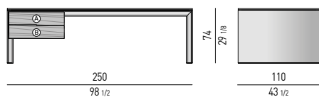
Foro passacavi | Cable hole cm 20x6
