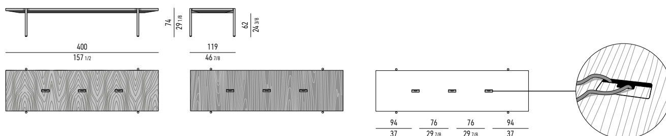
Foro passacavi | Cable hole cm 20x6
