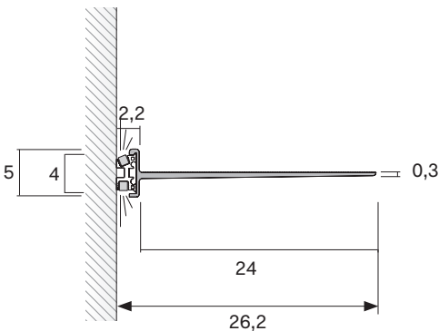
Mensola con luce LED su binario. Shelf with LED light on track.
