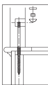
3008-10 NEWEL POST FASTENER 10-3/4"
