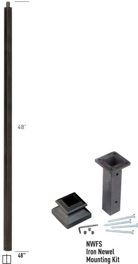
NWPL48 1-3/16" Plain Newel
