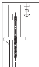
3008-10 NEWEL POST FASTENER 10-3/4" anchor bolt
