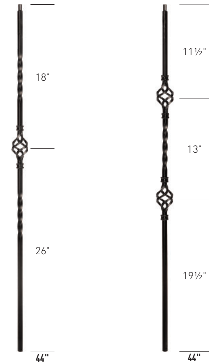
1BSK 44 One Basket
