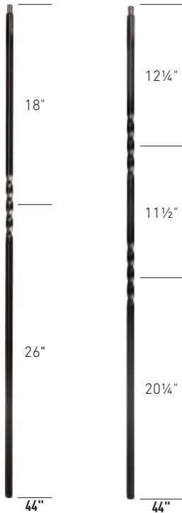
1TW 44 1/2" Single Twist 2TW 44 1/2" Double Twist
