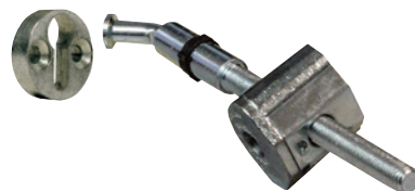
A3001SF — 2 Pack RAKE INSTALLATION ANGLED SLIPFIX ZIPBOLT™
