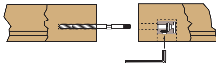
2 3001 SP — 2-Pack ZIPBOLT™
