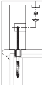
3070 THREADLOCK™ NEWEL POST FASTENER
