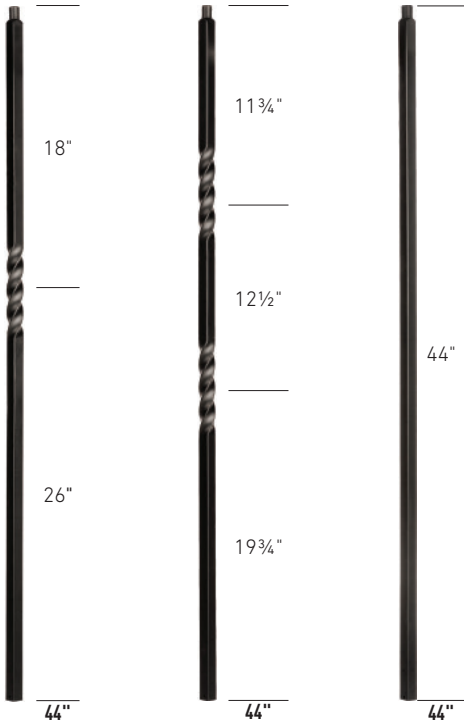
M1TW 44 3/4" Single Twist
