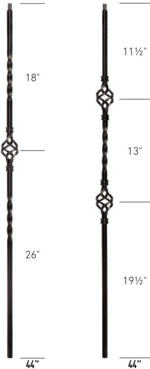
1BSK 44 1/2" Single Basket 2BSK 44 1/2" Double Basket
