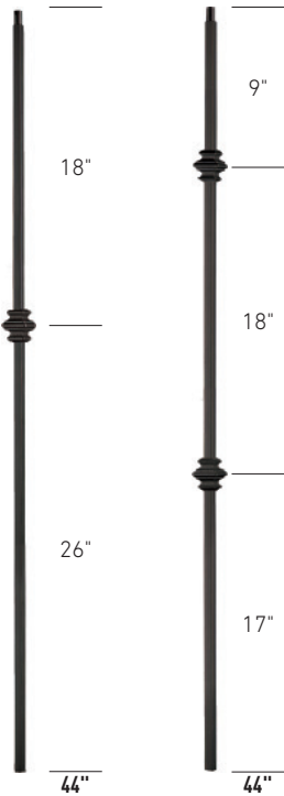
1KNU 44 1/2" Single Knuckle 2KNU 44 1/2" Double Knuckle
