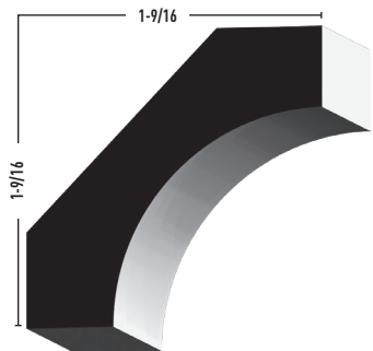
COVE CROWN
