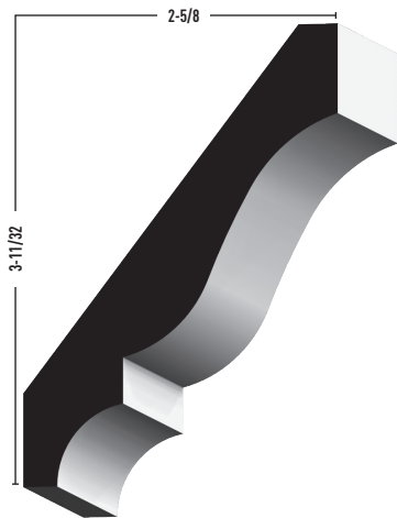
COLONIAL CROWN
