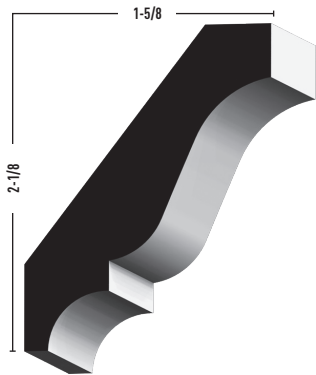
COLONIAL CROWN
