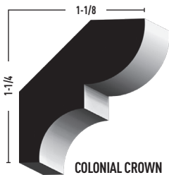
COLONIAL CROWN
