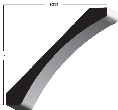
CONTEMPORARY CROWN
