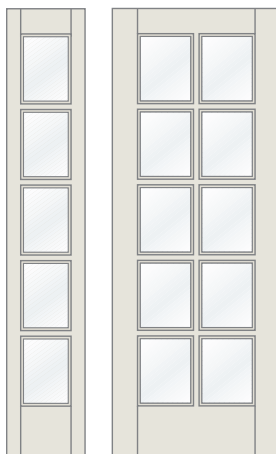
6-8: 5-Lite 6-8: 10 or 15-Lite 8-0: 6-Lite 8-0: 12 or 18-Lite
