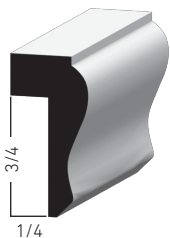
PLY CAP
