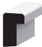
280 BACK BAND 11/16 x 1-1/8
