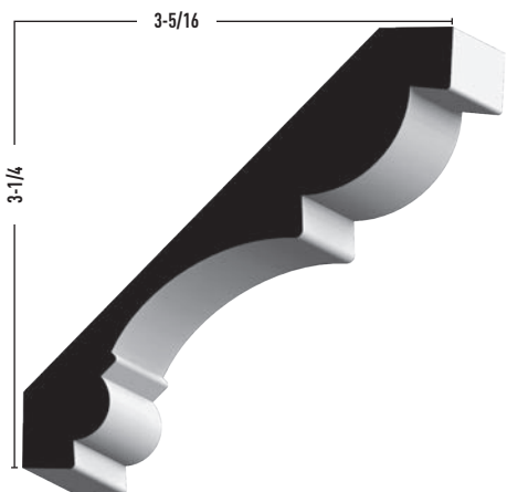
VICTORIAN CROWN
