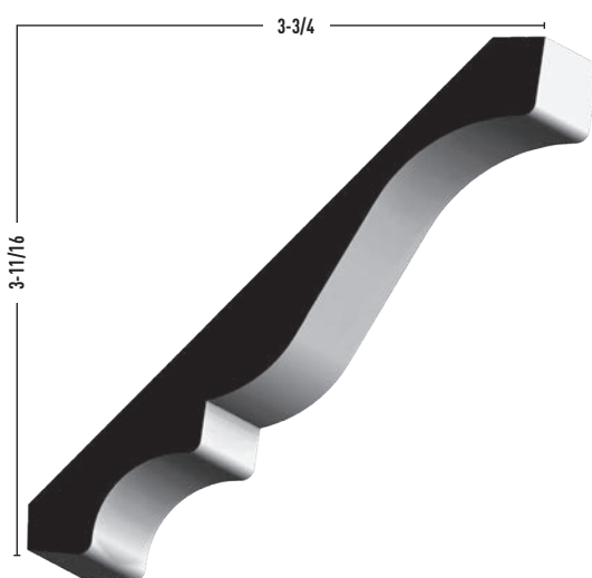
COLONIAL CROWN
