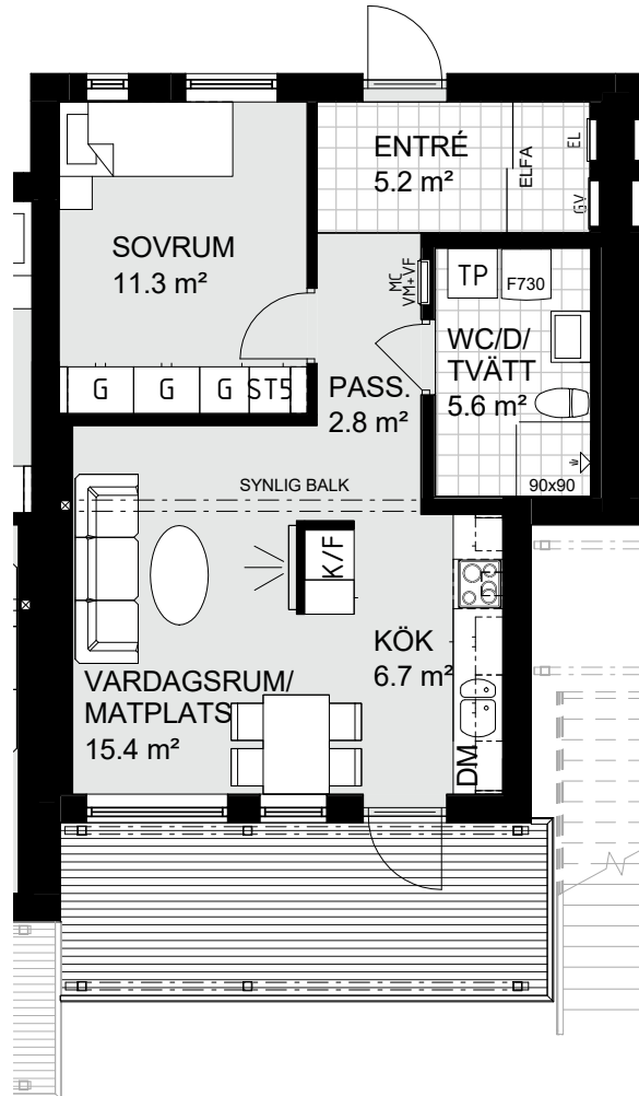
PLAN 1
