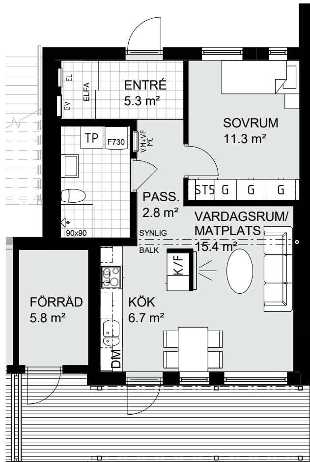
PLAN 1
