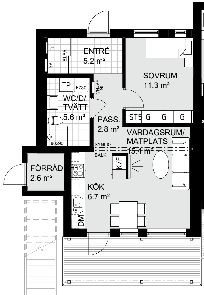
PLAN 1
