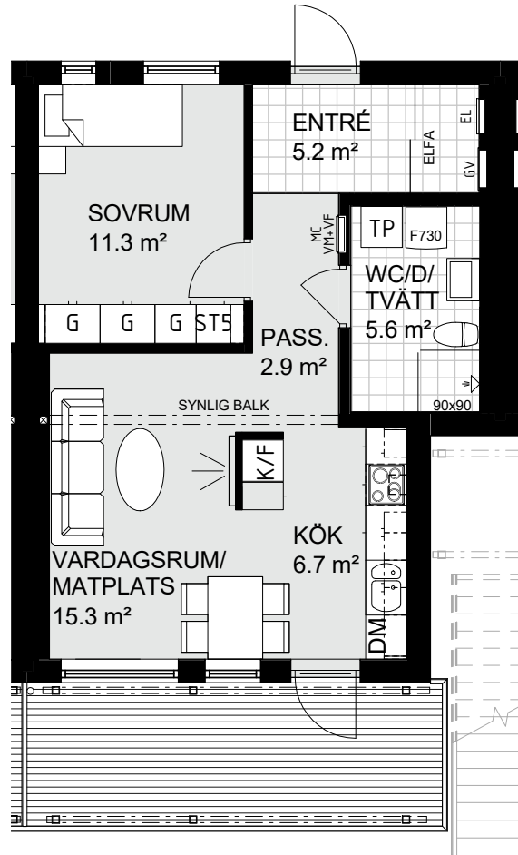
PLAN 1
