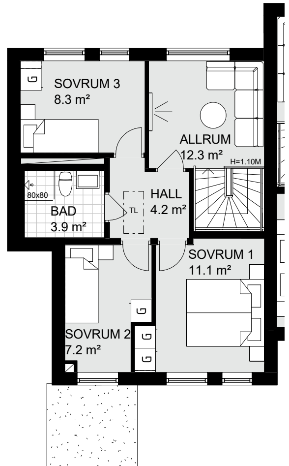
PLAN 3
