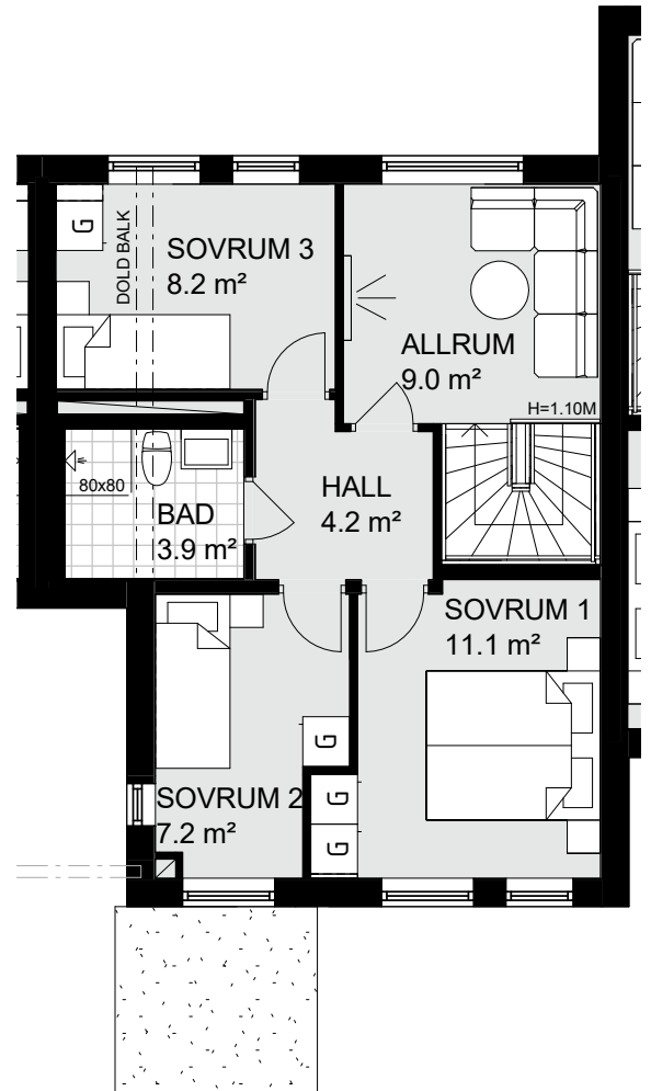
PLAN 3
