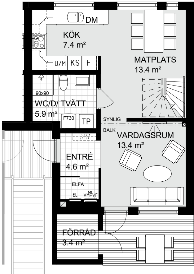
PLAN 2
