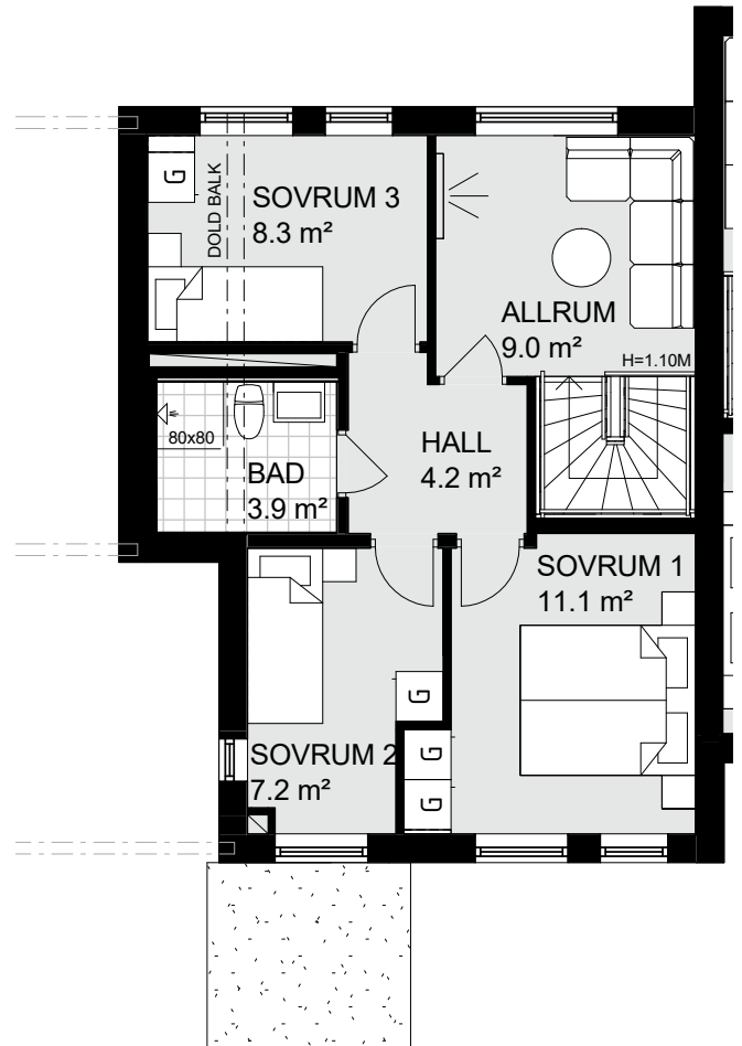
PLAN 3
