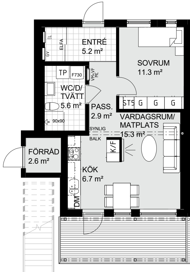
PLAN 1
