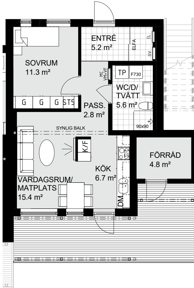
PLAN 1
