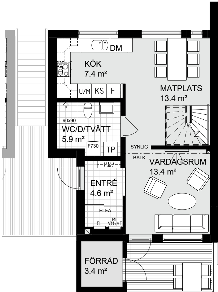
PLAN 2
