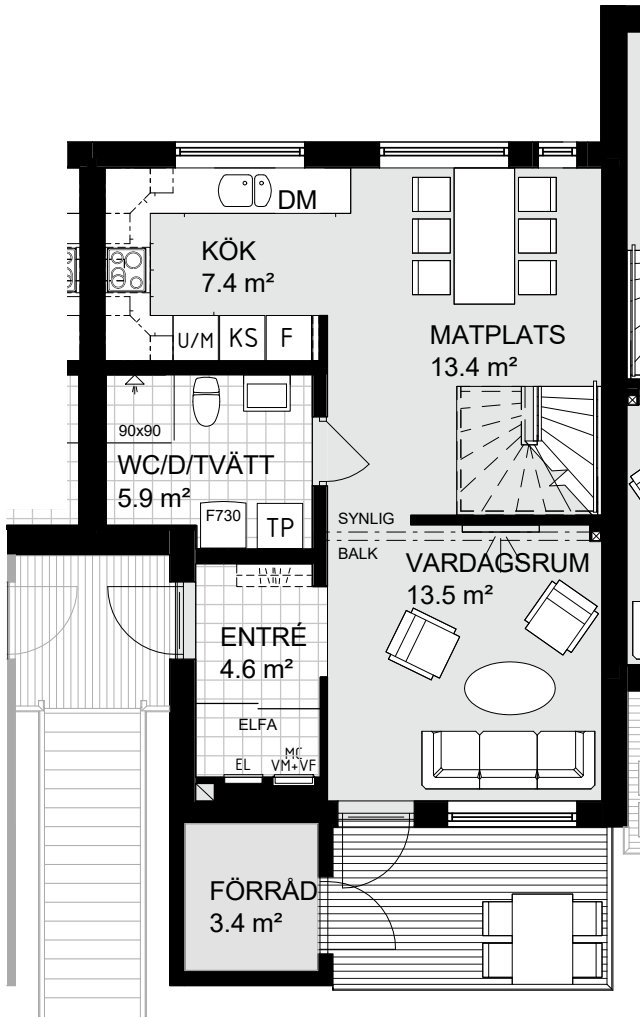
PLAN 2
