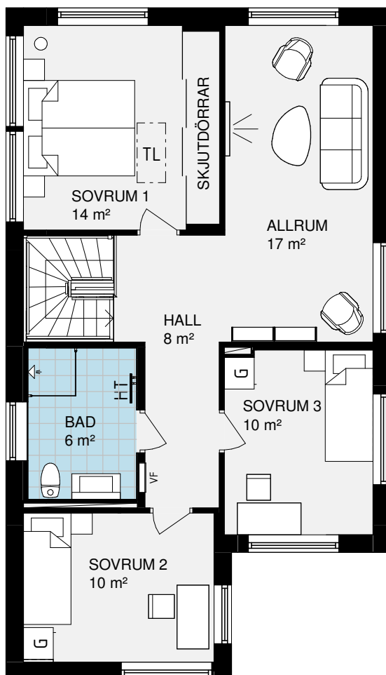
PLAN 2
