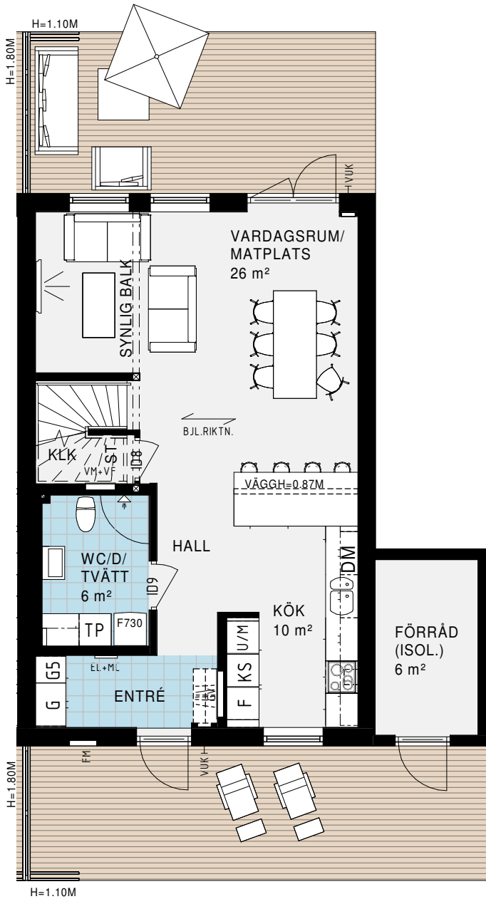
PLAN 1
