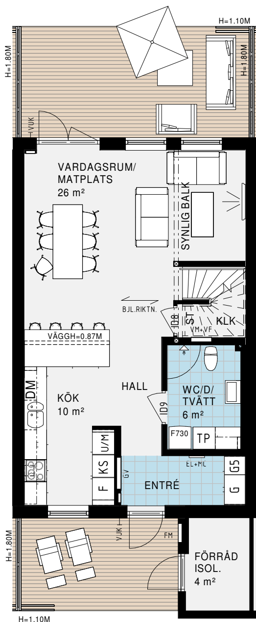
PLAN 1
