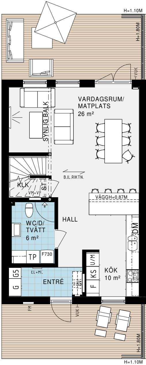
PLAN 1
