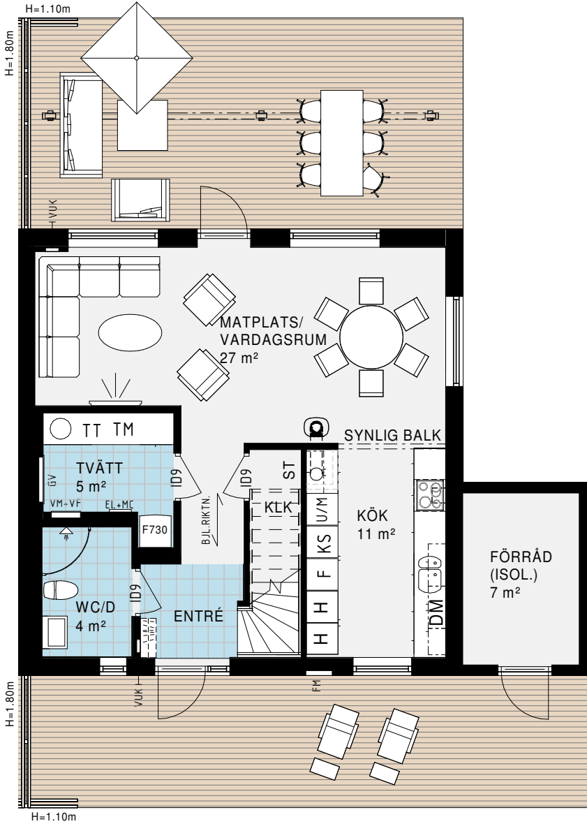
PLAN 1
