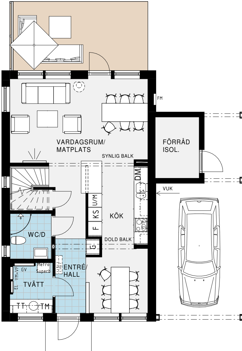
PLAN 1
