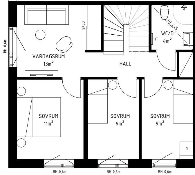
PLAN 2
