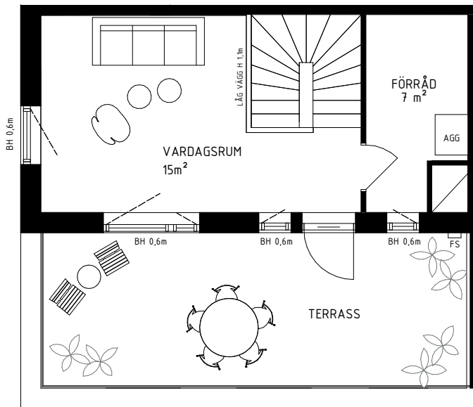
PLAN 3
