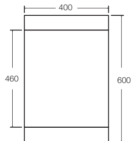
Mirror Cabinet Front Elevation
