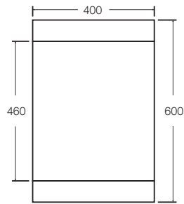
Mirror Cabinet Front Elevation
