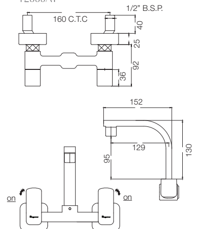
SINK MIXER T2335A1
