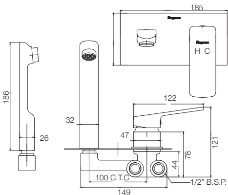
WALL MOUNTED BASIN MIXER T2376A1
