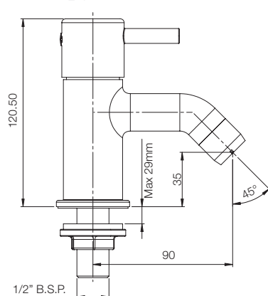
PILLAR COCK WITH AERATOR G3302A1
