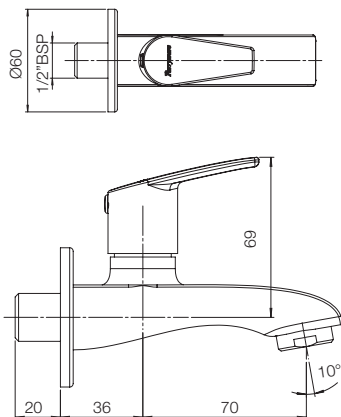
BIB COCK WITH AERATOR G4880A1
