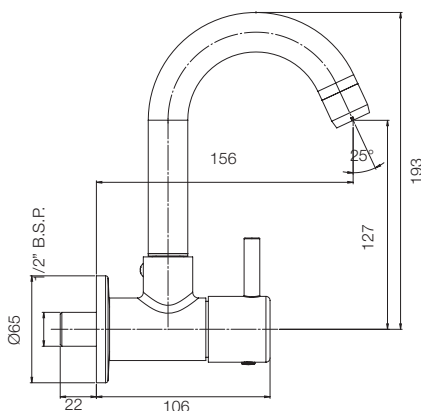
SINK COCK G3321A1
