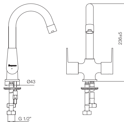
CENTER HOLE BASIN MIXER T1315A1
