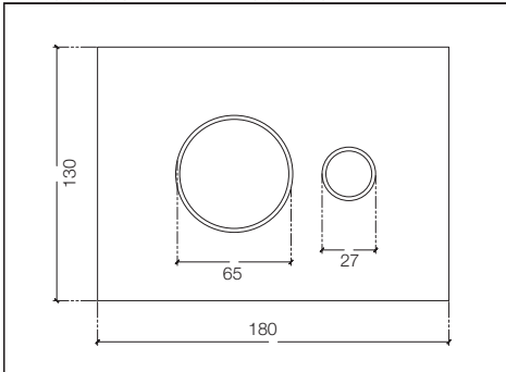
3-INLET DIVERTER UPPER TRIM T9966A1
