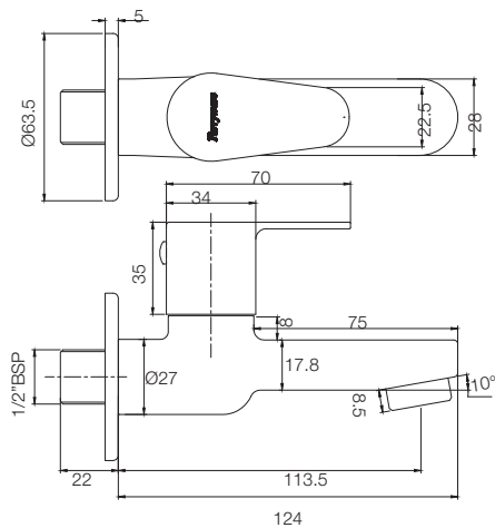
LONG BODY BIB COCK T5006A1 / C5006A1
