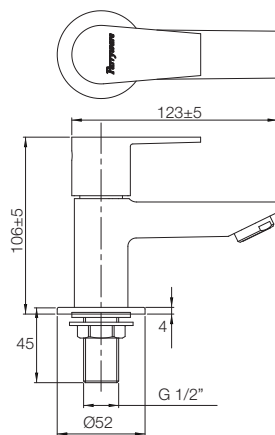
PILLAR COCK LONG NECK T131SA1
