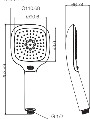
3-MODES. ONE TOUCH SWITCHING WITH HOSE + HOOK (125MM) T9817A1
