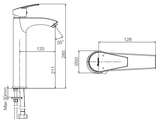
TALL BASIN MIXER G4846A1
