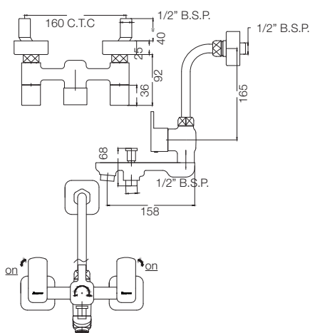
WALL MIXER 3 IN 1 T2317A1
