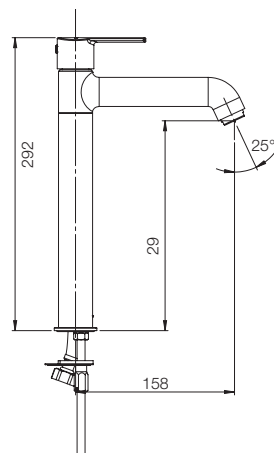
TALL PILLAR TAP G3164A1
