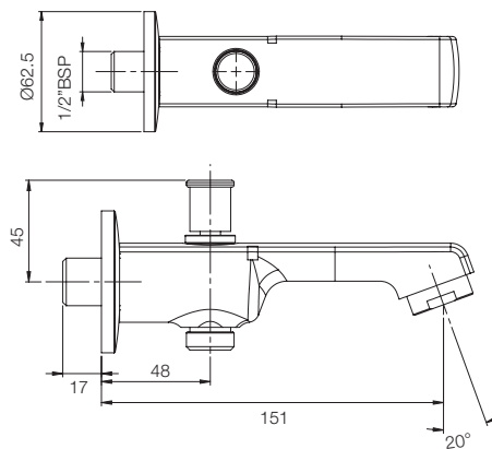
BATH SPOUT WITH DIVERTER G3128A1
