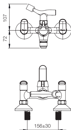
WALL MIXER WITH CRUTCH G272GA1
