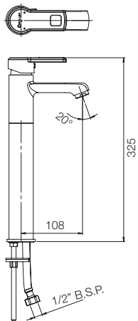
TALL BASIN MIXER G3946A1
