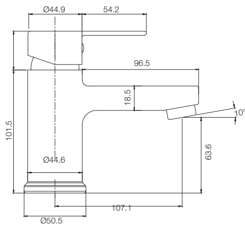
BASIN MIXER T5065A1
