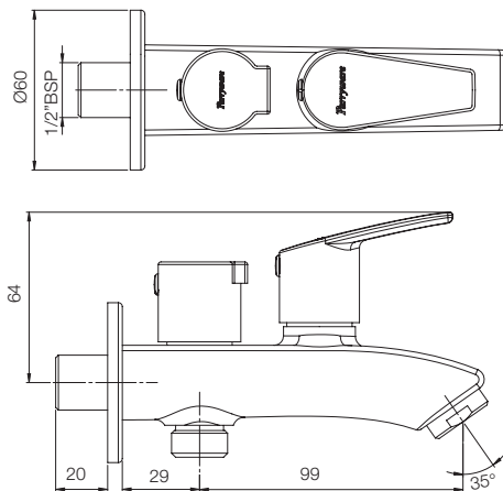
TWO WAY BIB COCK G4834A1
