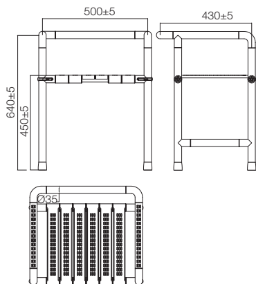
SHOWER SEAT MOVABLE T6811A1 (White)
