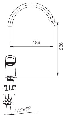
DECK MOUNTED SINK MIXER G2737A1
