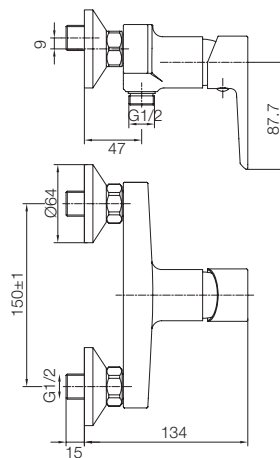
SHOWER MIXER T4958A5
