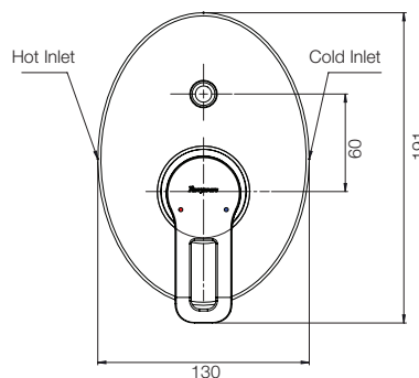
HI FLOW CON- CEALED DIVERT- ER UPPER TRIM G3885A1 HIGH FLOW/ DIVERTER BODY G4887A1
