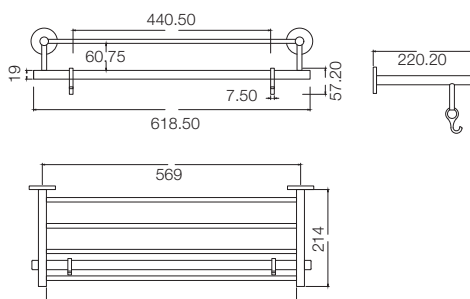
TOWEL RACK (24") T6008A1
