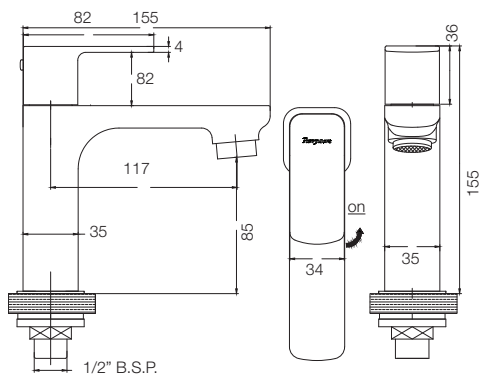
PILLAR COCK T2301A1
