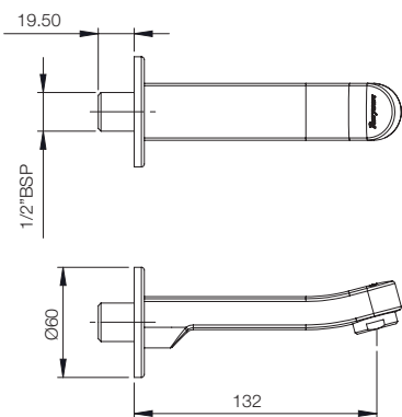
WALL SPOUT G2727A1
