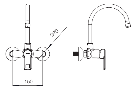
WALL MOUNTED SINK MIXER TOP OUTLET G391XA1
