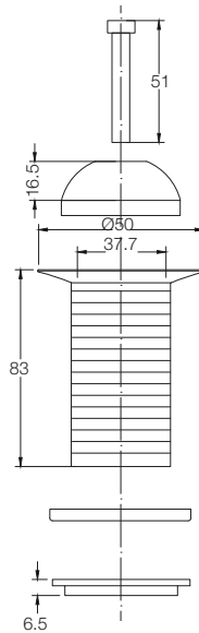
URINAL DOME WASTE COUPLING T9954A1
