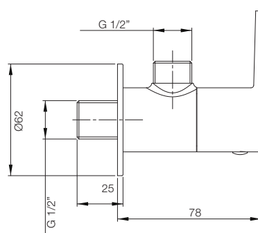
ANGLE VALVE WITH FLANGE T1372A1
