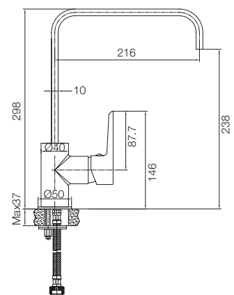
KITCHEN MIXER T4950A5
