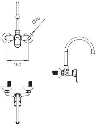
WALL MOUNTED SINK MIXER TOP OUTLET G271XA1
