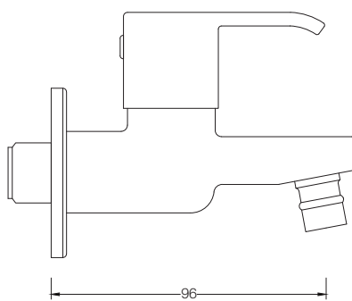
BIB COCK WITH NOZZLE G3879A1
