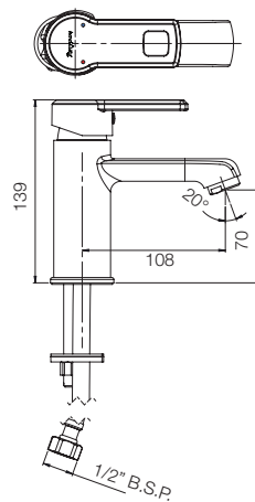
BASIN MIXER N G3965A1
