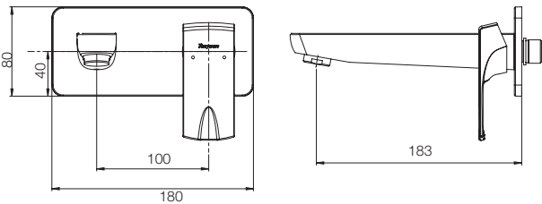
WALL MOUNT- ED BASIN MIXER UPPER TRIM G2376A1
