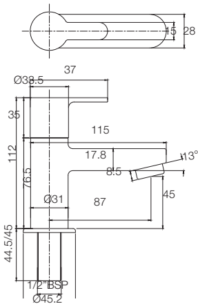
PILLAR COCK T4601A1/ G5201A1
