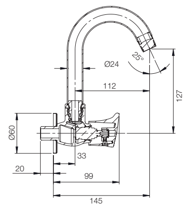
WALL MOUNTED SINK COCK G4721A1
