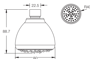
ALPHA SHOWER WITH SHOWER ARM (80MM) T9885A1
