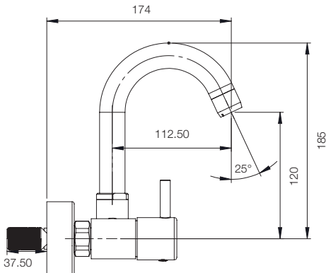
SINK MIXER G3335A1
