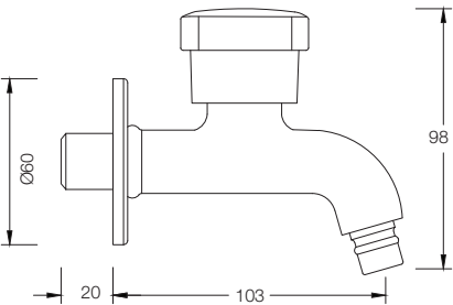
BIB COCK WITH NOZZLE G0279A1
