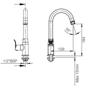
SWAN NECK PILLAR COCK G2703A1
