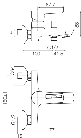
BATH MIXER T49I6A6
