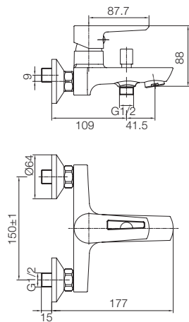
BATH MIXER T49I6A5
