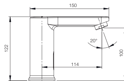
PILLAR COCK DC G541QA1
