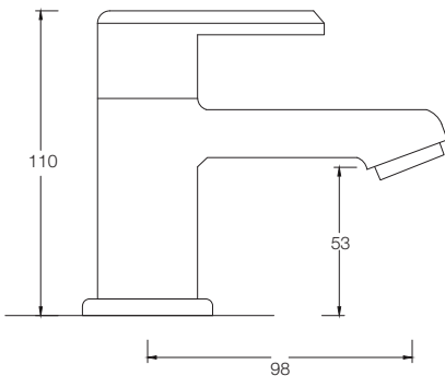
PILLAR COCK WITH AERATOR G3902A1
