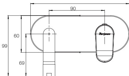
WALL MOUNTED PILLAR COCK UPPER TRIM G2796A1 COMPATIBLE WITH CONCEALED PILLAR COCK BODY G2797A1
