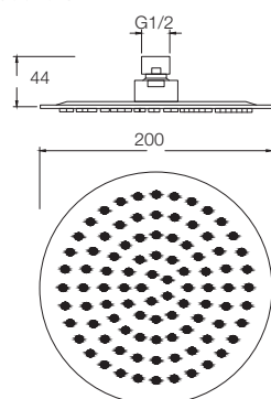
SS RAIN SHOWER WITHOUT ARM - ROUND (200MM) T9976A1
