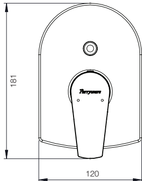
HIGH FLOW/CONCEALED DIVERTER UPPER TRIM G3285A1 HIGH FLOW/ DIVERTER BODY G4887A1
