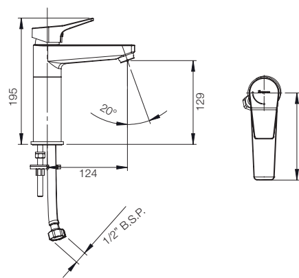
MEZZO BASIN MIXER G572AA1
