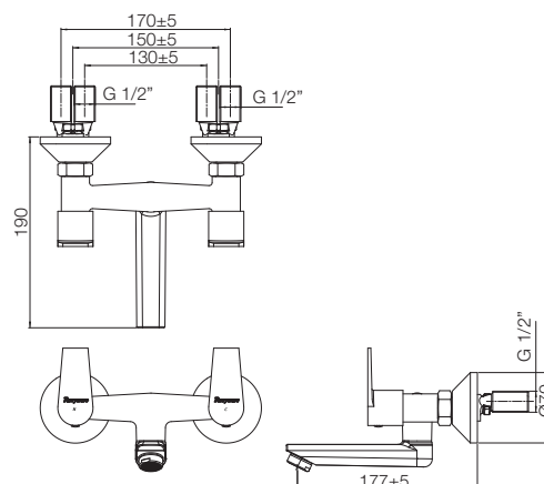
WALL MIXER NON TELEPHONIC T1341A1
