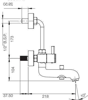
WALL MIXER 3-IN-1 G3317A1
