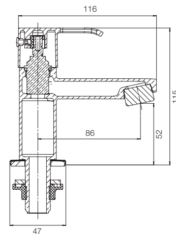
PILLAR COCK G3801A1
