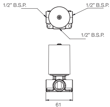
DEUSCH MIXER UPPER TRIM G311AA1 COMPATIBLE WITH CONCEALED SHOWER MIXER BODY G4257A1
