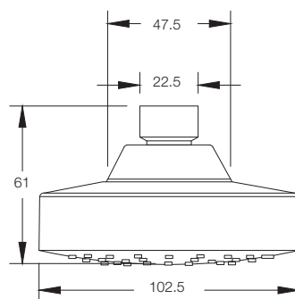
OVERHEAD SHOWER WITH ARM (100MM) T9808A1
