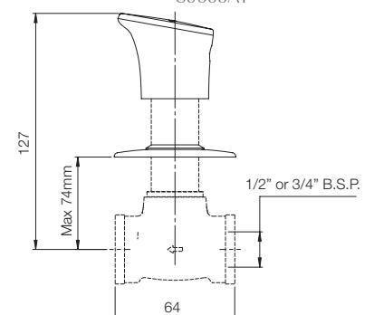
CONCEALED STOP COCK UPPER TRIM G4711A1 COMPATIBLE WITH CONCEALED BODY 1/2" & 3/4" G5052A1 G5053A1
