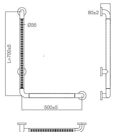
L SHAPE SUPPORT BAR (500MM) T6801A1 (White)
