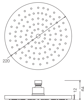
OVER HEAD SHOWER T4989A5
