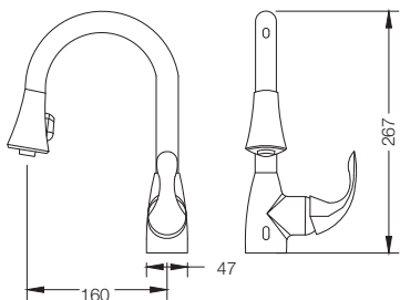
PULL OUT KITCHEN MIXER (WITH SENSOR) T4735A1
