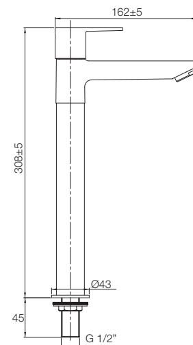
PILLAR COCK TALL BODY T1342A1
