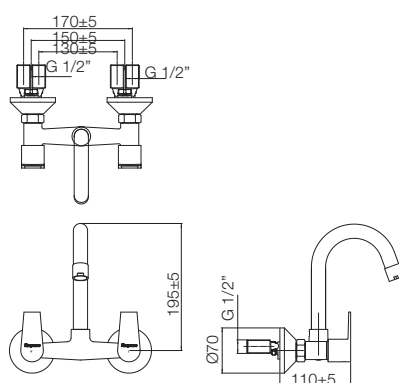
WALL MOUNTED SINK MIXER T1335A1
