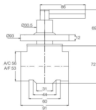
PLUTO CONTROL VALVE- 1.5 INCH T9894A3
