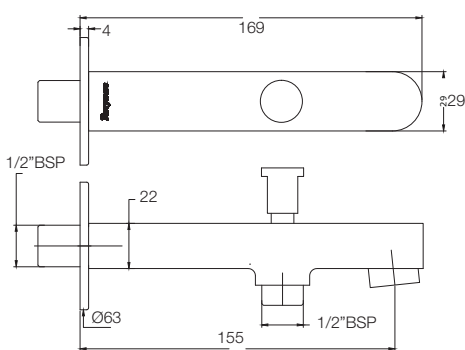
BATHSPOUT WITH DIVERTER T4627A1
