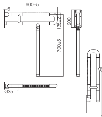
U SHAPED LIFT SUPPORT FIXED T6805A1 (White)
