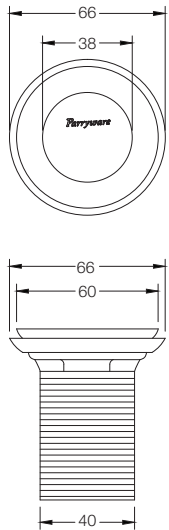
POP-UP WASTE COUPLING T9953A1
