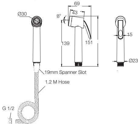
PLUTO HEALTH FAUCET WITH HOSE + HOOK E8384A1
