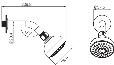
SINGLE FLOW OVERHEAD SHOWER WITH SS SHOW- ER ARM & WALL FLANGE (80MM) T9984A1
