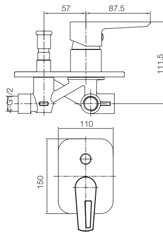
CONCEALED BATH MIXER T4926A6
