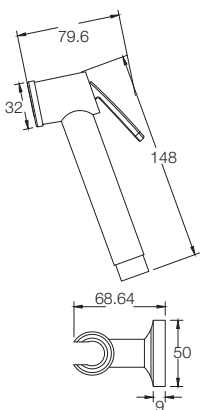
CARDIFF PRO WITH HOSE + HOOK T9875A1
