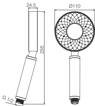
2 MODES, SELF CLEANING, HOSE + HOOK T9872A1
