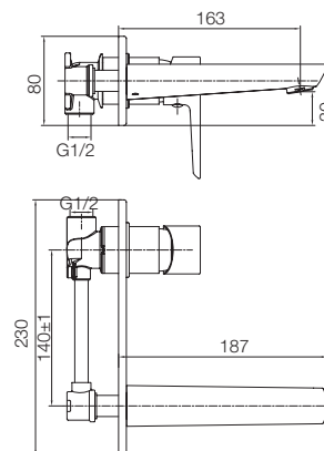
CONCEALED BASIN MIXER T4956A6
