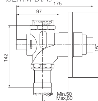
CONCEALED DUAL FLUSH VALVE (40MM DIA.) CONCEALED DUAL FLUSH VALVE (32MM DIA.)
