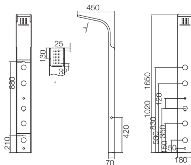
VERVE WITH CASCADE WATERFALL / RAIN SHOWER AND 4 BODY JETS C884099
