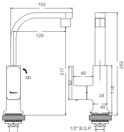
SWAN NECK PILLAR TAP T2303A1
