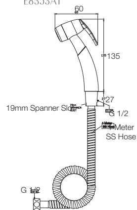
CORAL NEO WITH HOSE + HOOK E8353A1
