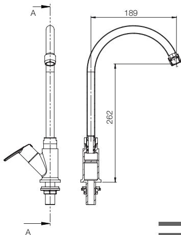
DECK MOUNTED SINK COCK G4820A1
