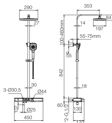
RAIN & HS (ADJUSTABLE) THERMOSTAT T9822A1
