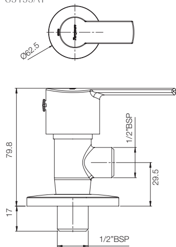
ANGLE VALVE WITH WALL FLANGE G3153A1
