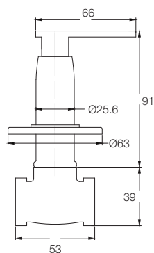
CONCEALED STOP COCK (WITH BODY) - 20MM T1912A1
