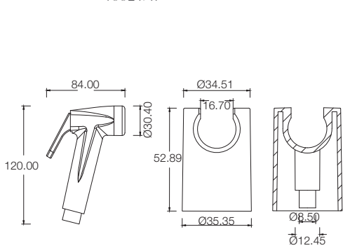
UNO WITH HOSE + HOOK T9921A1
