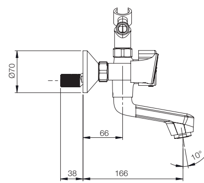
WALL MIXER WITH CRUTCH G4719A1
