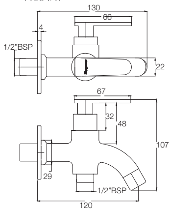
TWO WAY BIB COCK T1934A1
