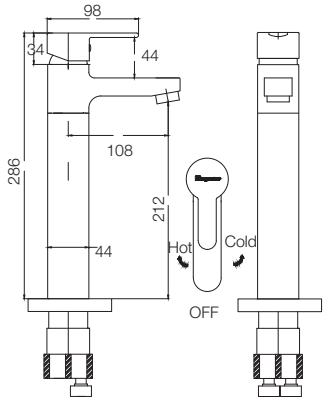
TALL BODY BASIN MIXER T4646A1
