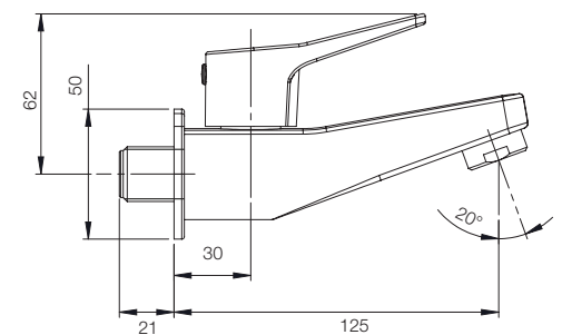
LONG BODY BIB COCK G5706A1
