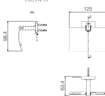
PAPER HOLDER WITH COVER T6514A1
