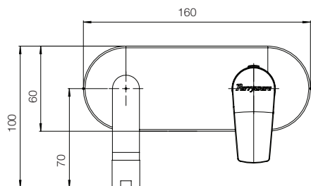
BASIN MIXER UPPER TRIM G3276A1 COMPATIBLE WITH CONCEALED BODY BASIN MIXER G9002A1
