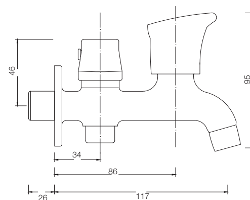
TWO WAY BIB COCK WITH AERATOR G471ZA1
