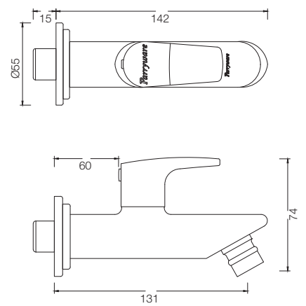
BIB COCK WITH NOZZLE G3279A1
