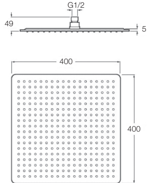
SS RAIN SHOWER WITHOUT ARM - SQUARE (400MM) T9990A1
