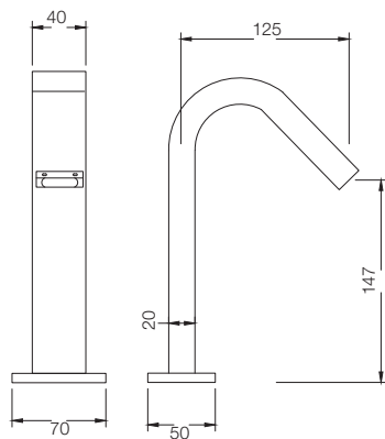
SOAP DISPENSER FAUCET T4788A1
