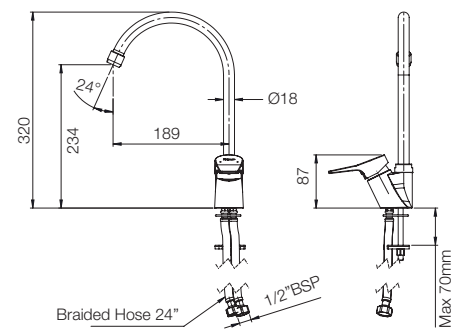
DECK MOUNTED SINGLE LEVER SINK MIXER G571GA1
