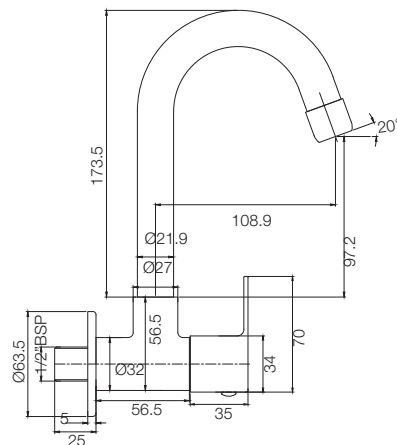
WALL MOUNTED SINK COCK T5021A1
