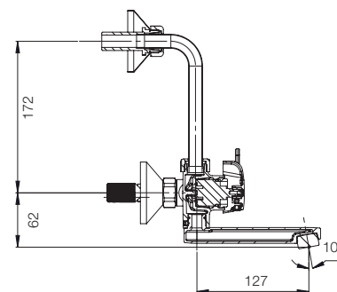
ANGLE VALVE (HEAVY) G4707A1
