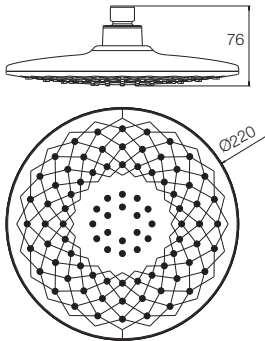
SELF CLEANING BLACK FACEPLATE (220MM) T9837A1
