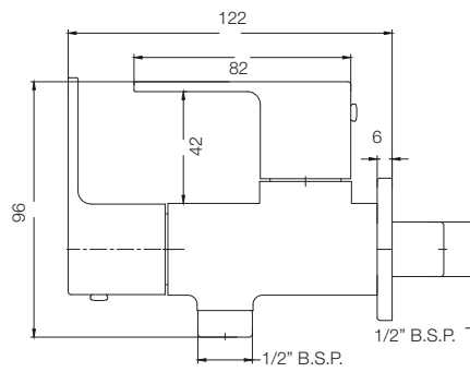
TWO WAY ANGLE VALVE T2343A1
