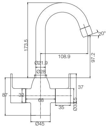
BASIN MIXER (CENTER HOLE) T4614A1
