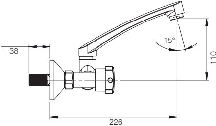
WALL MOUNTED SINK MIXER G0235A1
