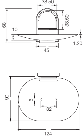
SOAP DISH T6503A1
