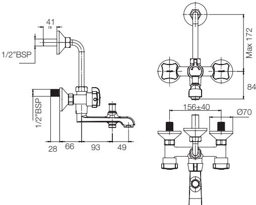
WALL MIXER 3-IN-1 G022FA1
