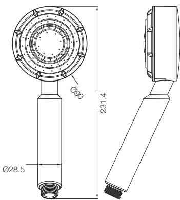
CENTER LED HAND SHOWER: HOSE + HOOK T9855A1
