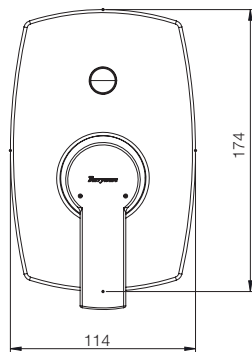
ULTRA HIGH FLOW DIVERTER UPPER TRIM G3185A1 HIGH FLOW DIVERTER BODY G4887A1
