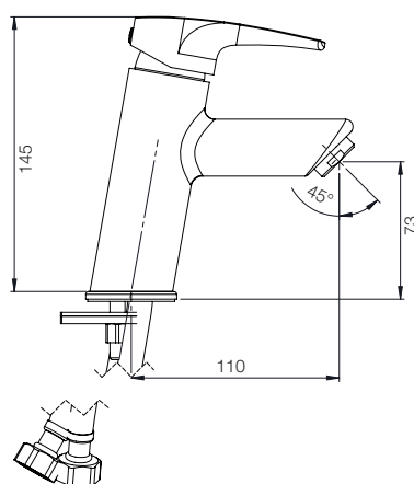
BASIN MIXER G3265A1
