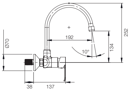
WALL MOUNTED SINK MIXER- TOP OUTLET G3835A1
