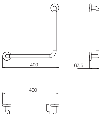
HAND GRIP 90 RIGHT T6607A1
