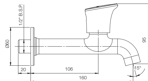
LONG BODY BIB COCK G4706A1
