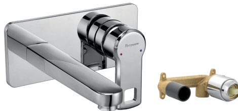
BASIN MIXER UPPER TRIM G3976A1 COMPATIBLE WITH CONCEALED BODY BASIN MIXER G9002A1
