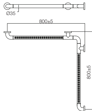
L SHAPE SUPPORT BAR CORNER RAIL (800MM) T6803A1 (White)
