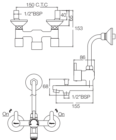
WALL MIXER 3-IN-1 T4617A1
