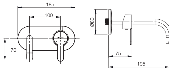
WALL MOUNT- ED BASIN MIXER UPPER TRIM G5276A1
