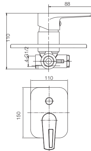
CONCEALED SHOWER MIXER T4957A6
