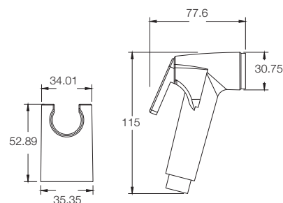
CASA HEALTH FAUCET WITH HOSE + HOOK T9887A1
