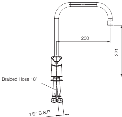
DECK MOUNTED SINK MIXER G4837A1
