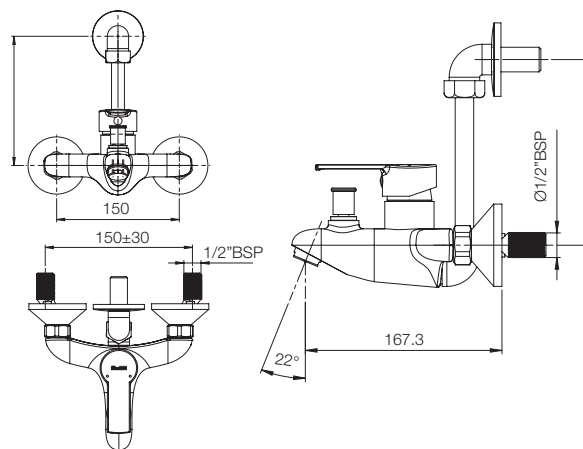
SINGLE LEVER WALL MIXER WITH BEND G3154A1
