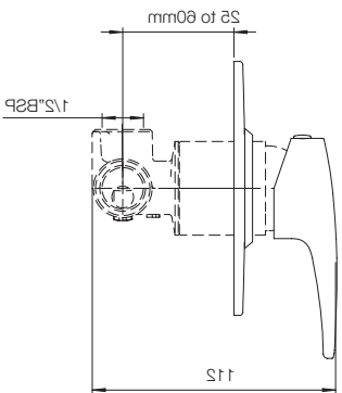
DEUSCH UPPER TRIM G321AA1 COMPATIBLE WITH CONCEALED SHOWER MIXER BODY G4257A1
