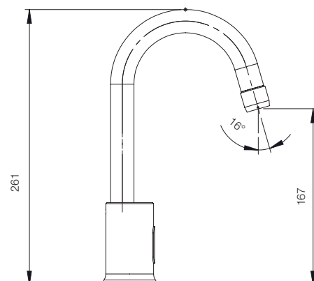
TALL PILLAR COCK AC/DC G541UA1
