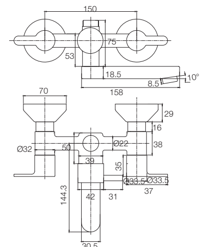
WALL MIXER 2-IN-1 T4616A1/G5216A1
