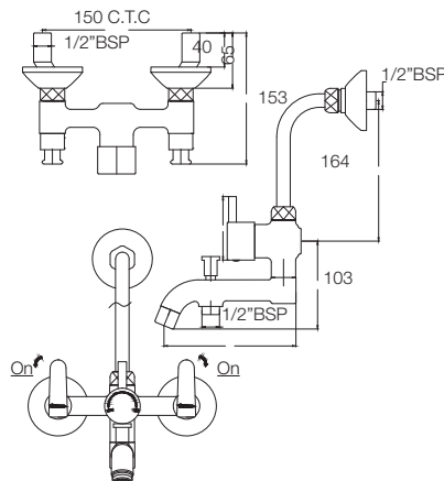
WALL MIXER 3 IN 1 T1917A1
