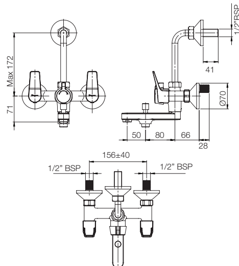
WALL MIXER 3-IN-1 G572FA1
