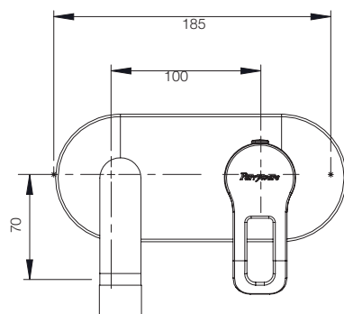
CONCEALED BASIN MIXER UPPER TRIM G3876A1 COMPATIBLE WITH CONCEALED BODY BASIN MIXER G9002A1
