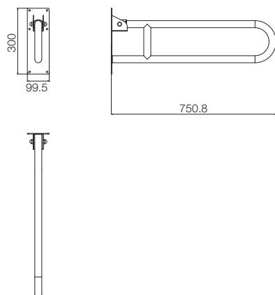
HINGED GRAB RAIL T6608A1
