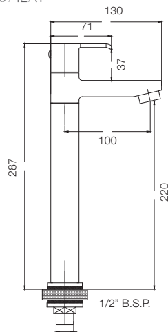
TALL PILLAR COCK T0742A1
