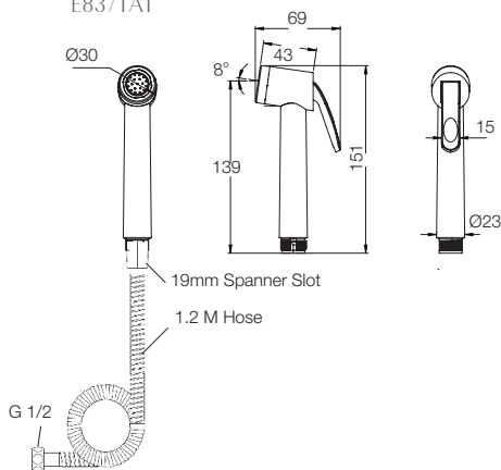
OVALO SELF CLEANING WITH SS HOSE + HOOK E8371A1
