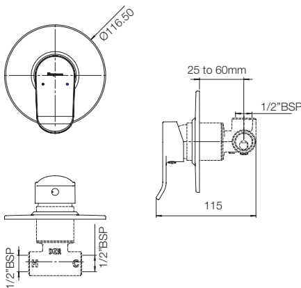
DEUSCH MIXER UPPER TRIM G271AA1 COMPATIBLE WITH CONCEALED SHOWER MIXER BODY G4257A1
