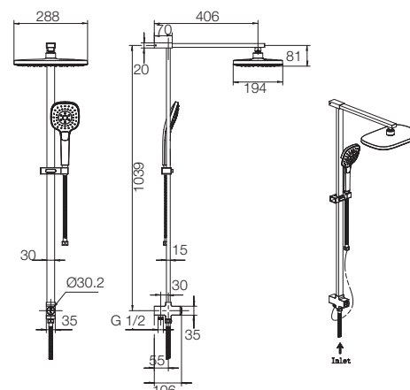
RAIN & HS (FIXED) T9821A1
