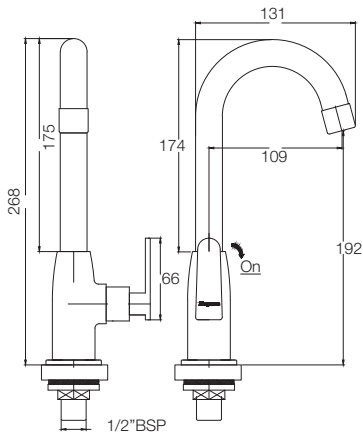
SWAN PILLAR TAP T1903A1
