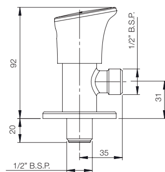
ANGLE VALVE (LIGHT) G4753A1
