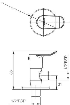
ANGLE VALVE G2707A1
