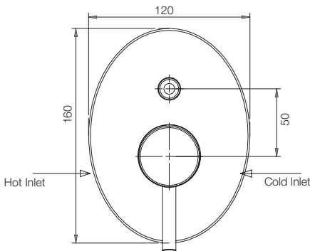
CONCEALED DIVERTER UPPER TRIM G0650A1
