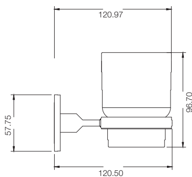
TUMBLER HOLDER T6004A1
