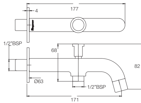
BATH SPOUT WITH DIVERTER T1928A1
