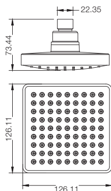
EASY CLEANING SHOWER WITH SHOWER ARM (125MM) T9850A1
