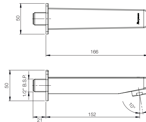
WALL SPOUT G5727A1
