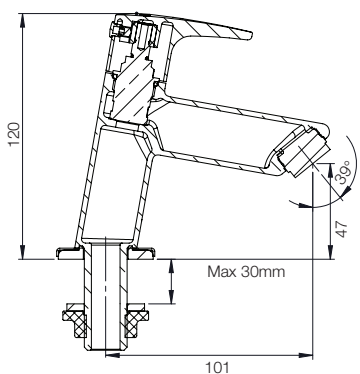
PILLAR TAP G3266A1
