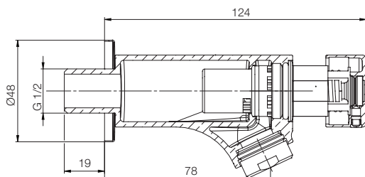
BIB COCK AUTO CLOSING SYSTEM G2056A1
