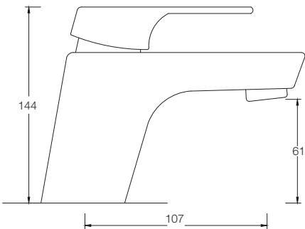
BASIN MIXER N G2365A1
