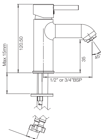
SINGLE LEVER BASIN MIXER (COLD START) G3314A1
