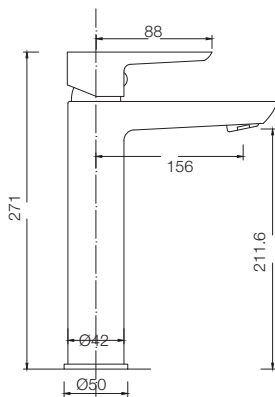
TALL BASIN MIXER T4946A5
