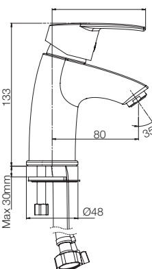
BASIN MIXER G4814A1
