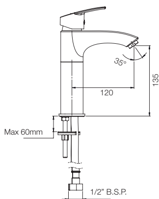
HIGH NECK BASIN MIXER (MEDIUM) G4863A1
