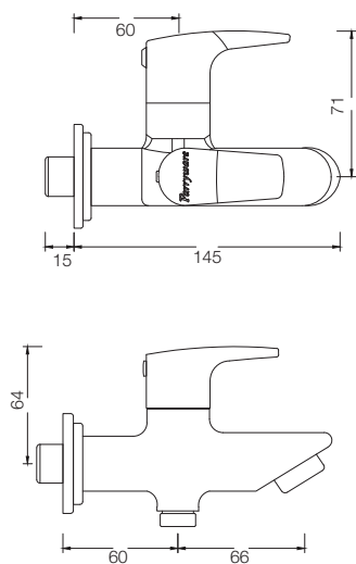
TWO WAY BIB COCK G3234A1
