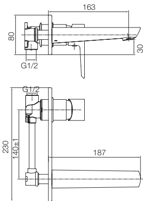
BASIN MIXER T4956A5
