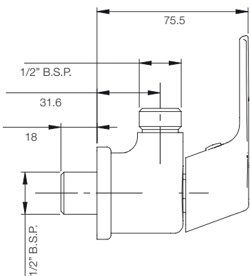
ANGLE VALVE WITH WALL FLANGE G2307A1
