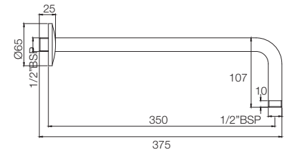
WALL MOUNTED 15" SHOWER ARM T9802A1
