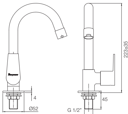
PILLAR COCK SWANNECK LEFT HAND T1303A1
