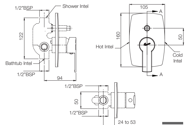
CONCEALED DIVERTER UPPER TRIM G3150A1 COMPATIBLE WITH CONCEALED DIVERTER BODY G5051A1
