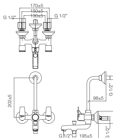
WALL MIXER 3-IN-1 T1317A1
