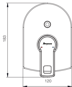
CONCEALED DIVERTER UPPER TRIM G3950A1
