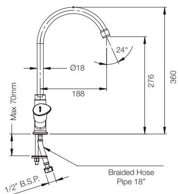
DECK MOUNTED SINK MIXER G4750A1
