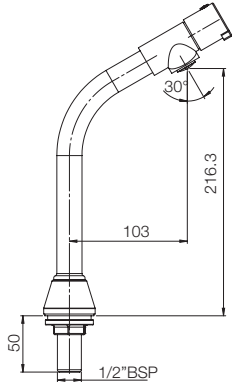
SMART HIGH NECK STANDALONE PILLAR TAP G3764A1
