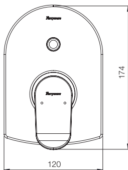
ULTRA HIGH FLOW DIVERTER UPPER TRIM G2785A1 HIGH FLOW DIVERTER BODY G4887A1
