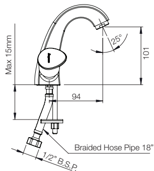
BASIN MIXER G4715A1
