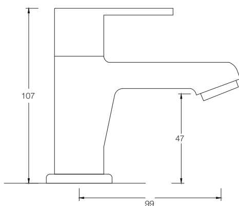
PILLAR COCK WITH AERATOR G3102A1
