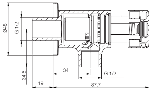
URINAL VALVE AUTO CLOSING SYSTEM G2007A1
