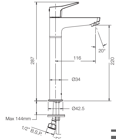
TALL PILLAR COCK WITH AERATOR G5702A1
