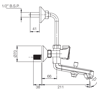
WALL MIXER 3-IN-1 G4717A1
