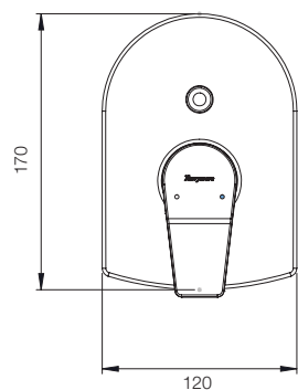
CONCEALED DIVERTER UPPER TRIM G5750A1 COMPATIBLE WITH CONCEALED DIVERTER BODY G5051A1
