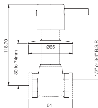
CONCEALED STOP COCK UPPER TRIM G3351A1 COMPATIBLE WITH CONCEALED BODY 1/2" & 3/4" G5052A1 G5053A1
