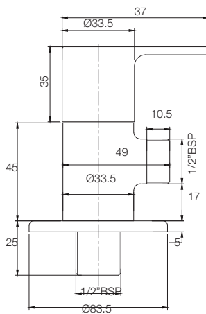
ANGLE VALVE T4607A1/ G5207A1
