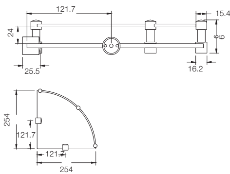
CORNER SHELF T6010A1
