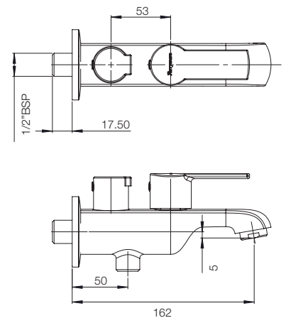
TWO-WAY BIB COCK WITH TWO KNOBS G3181A1
