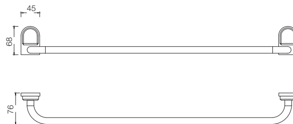
TOWEL RAIL (24") T6001A1
