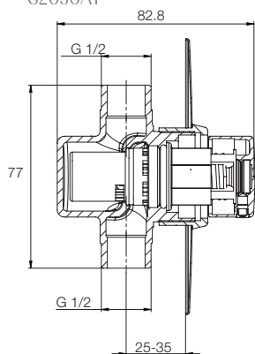
AUTO CLOSING CONCEALED URINAL FLUSH VALVE G2030A1
