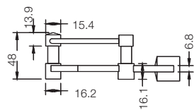
STRAIGHT SHELF T6009A1
