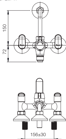
WALL MIXER 2-IN-1 G272EA1
