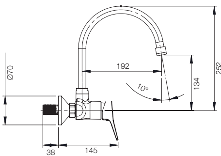
WALL MOUNTED SINK MIXER TOP OUTLET G571XA1
