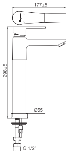
TALL BODY BASIN MIXER T1346A1
