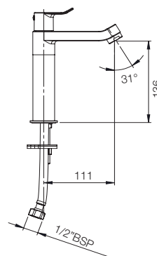
MEZZO PILLAR COCK WITH AERATOR G2766A1
