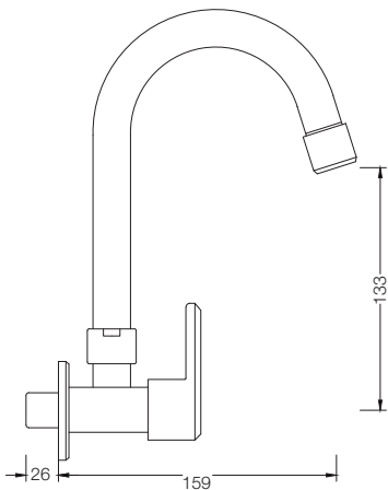
SINK COCK G3921A1
