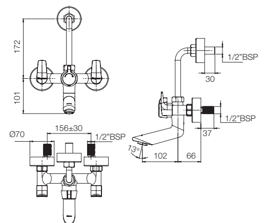
WALL MIXER 2-IN-1 G3216A1
