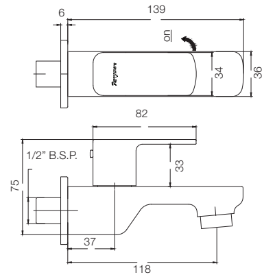
LONG BODY BIB COCK T2306A1
