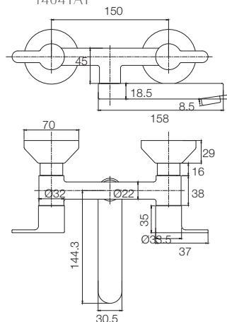
WALL MIXER NON TELEPHONIC T4641A1
