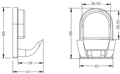
TWIN ROBE HOOK T6905A1
