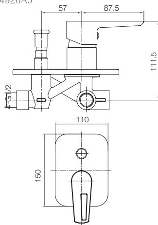
CONCEALED BATH MIXER T4926A5
