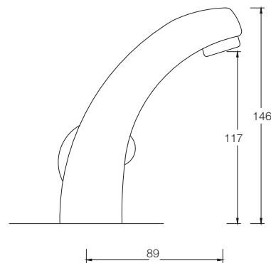
SWAN NECK PILLAR COCK G4768A1
