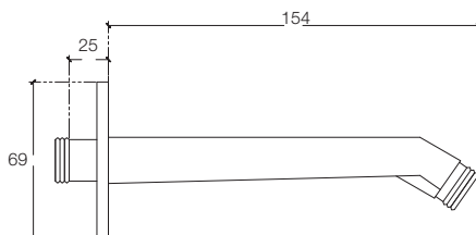
SQUARE SHOWER ARM 7" T9955A1
