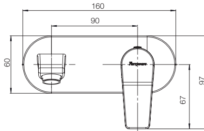
WALL MOUNTED CONCEALED PILLAR TAP UPPER TRIM G5796A1 COMPATIBLE WITH CONCEALED PILLAR COCK BODY G2797A1
