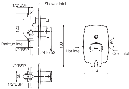
CONCEALED DIVERTER UPPER TRIM G2350A1
