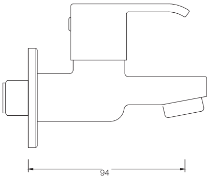
BIB COCK G3804A1
