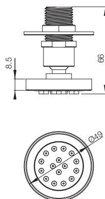
SOMA - ROUND BODY JET T9879A1
