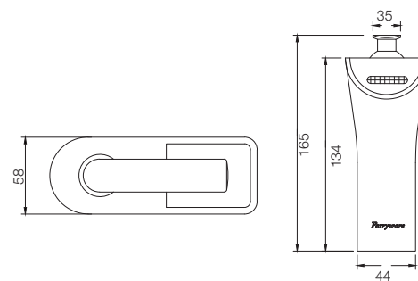
BASIN MIXER T171LA1
