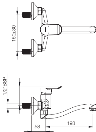
WALL MOUNTED SINK MIXER G2735A1
