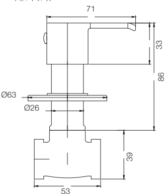
CONCEALED STOP COCK-1/2" WITH BODY T0711A1
