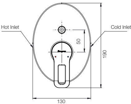
CONCEALED DIVERTER UPPER TRIM G3850A1 COMPATIBLE WITH CONCEALED DIVERTER BODY G5051A1
