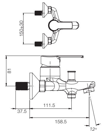
SINGLE LEVER WALL MIXER G3118A1
