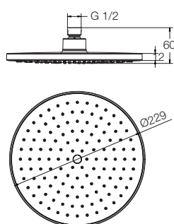
CHROME COMFORT FLOW SHOWER (230MM) T9840A1
