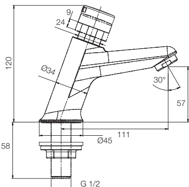
PILLAR COCK AUTO CLOSING SYSTEM G2013A1
