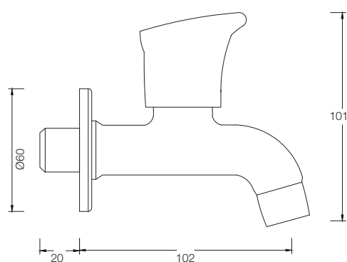
BIB COCK WITH AERATOR G4780A1
