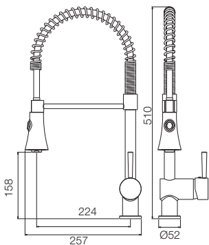
PLUTO PULL OUT KITCHEN MIXER T9895A1
