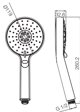
3 MODES. SOLID BLACK. HOSE + HOOK T9866A1
