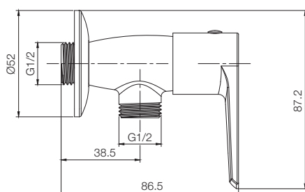
ANGLE VALVE T4907A5
