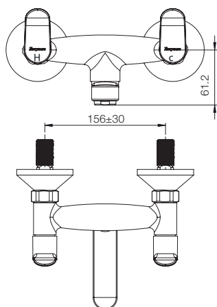
WALL MIXER NON TELEPHONIC G2741A1
