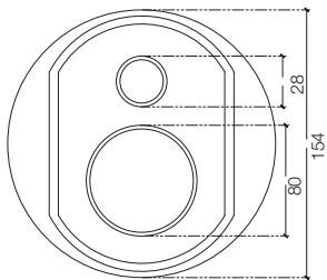
HIGH FLOW/ DIVERTER UPPER TRIM T9972A1 HIGH FLOW/ DIVERTER BODY G4887A1
