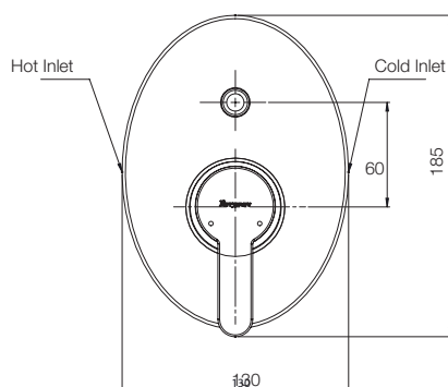
CONCEALED HI FLOW DIVERTER UPPER TRIM G5285A1
