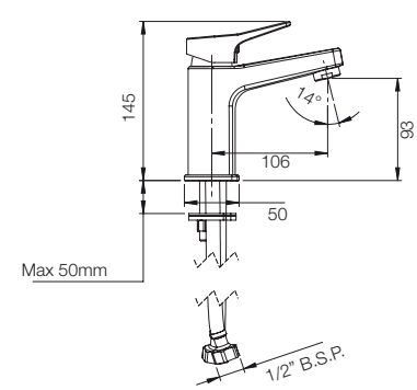
BASIN MIXER G5714A1
