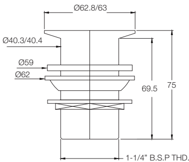
ALPHA WASTE COUPLING (80MM) (12 PIECES) T9882A1
