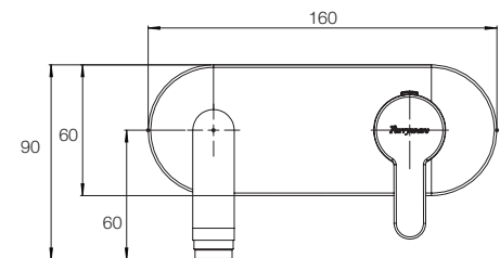
WALL MOUNTED PILLAR COCK UPPER TRIM G5296A1
