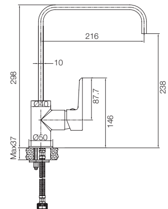
KITCHEN MIXER T4950A6
