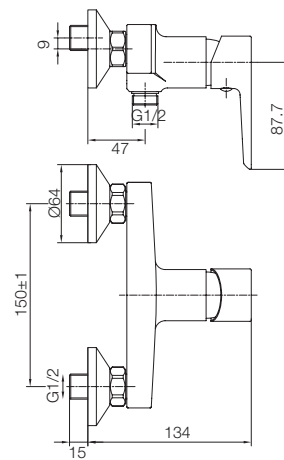
SHOWER MIXER T4958A6
