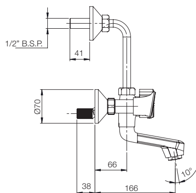
WALL MIXER 2-IN-1 G4716A1
