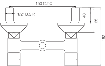
WALL MIXER NON TELEPHONIC T0741A1
