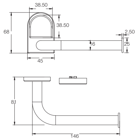
PAPER HOLDER T6906A1
