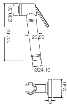
CARDIFF WITH SS HOSE + HOOK (BRASS) T9941A1
