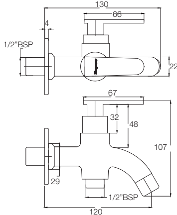
BIB COCK T1904A1
