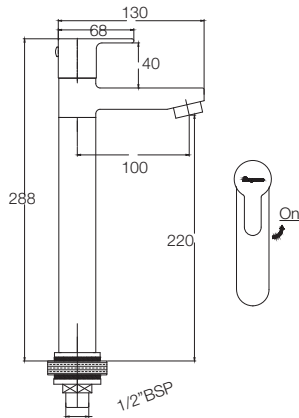
TALL PILLAR COCK T4642A1
