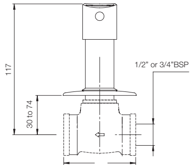
UPPER TRIM (CSC 1/2" & 3/4") G3283A1 COMPATIBLE WITH CONCEALED BODY 1/2" & 3/4" G5052A1 G5053A1
