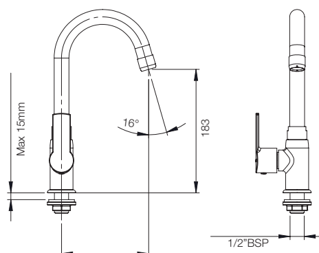
SWAN NECK PILLAR COCK G3103A1
