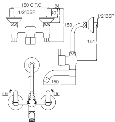
WALL MIXER 2 IN 1 T1916A1
