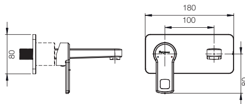
BASIN MIXER UPPER TRIM G3976A1 COMPATIBLE WITH CONCEALED BODY BASIN MIXER G9002A1
