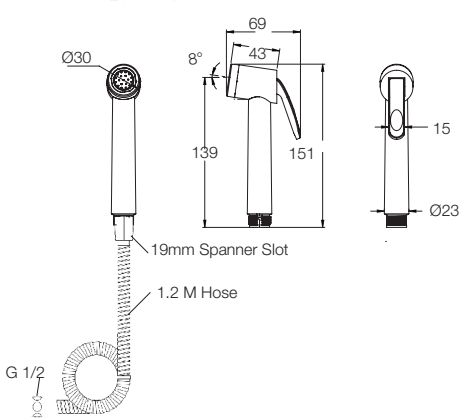
PRIMO HEALTH FAUCET WITH HOSE + HOOK E8383A1
