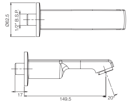
BATH SPOUT G3127A1
