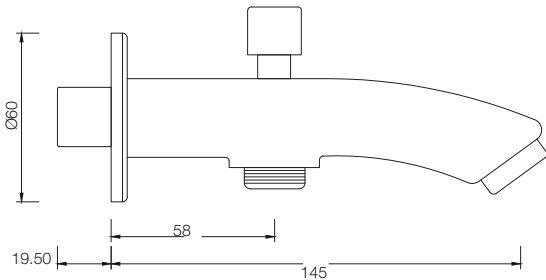
WALL SPOUT WITH DIVERTER G4828A1
