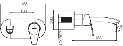
WALL MOUNTED BASIN MIXER UPPER TRIM G4876A1 COMPATIBLE WITH CONCEALED BODY BASIN MIXER G9002A1
