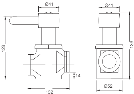
FLUSH COCK – LEVER TYPE (WORKS WELL FOR LOW PRESSURE) T3306A1
