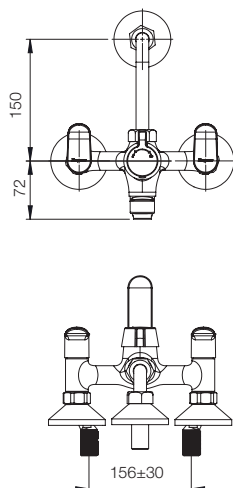
WALL MIXER 3-IN-1 G272FA1
