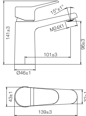
NIGHTLIFE BASIN MIXER T4915A5
