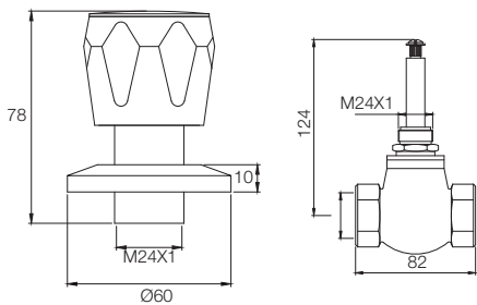
CORAL EXPOSED PART OF FLUSH COCK (SLEEVE/ HANDLE/FLANGE) T9825A1
