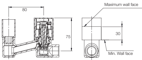
WALL MOUNT- ED BASIN TAP UPPER TRIM (PRESSMATIC) G2076A1 COMPATIBLE WITH WALL MOUNTED BASIN TAP BODY (PRESSMATIC) G2078A1
