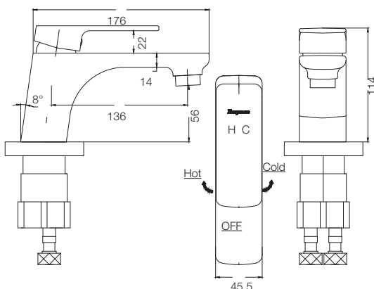
SINGLE LEVER BASIN MIXER 4" T2365A1
