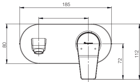
WALL MOUNTED BM UPPER TRIM G5776A1 COMPATIBLE WITH CONCEALED BODY BASIN MIXER G9002A1
