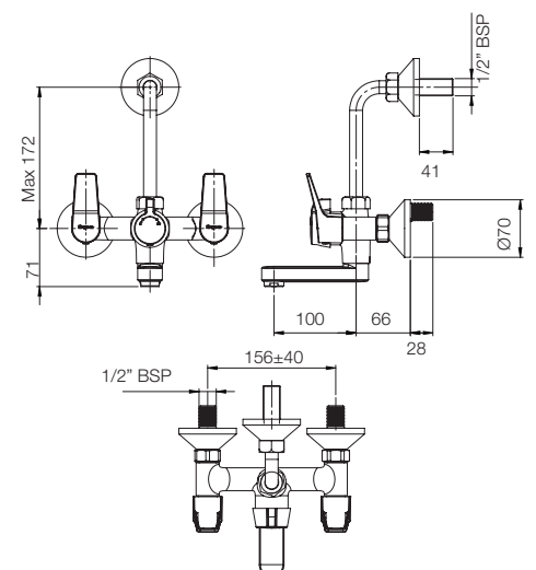
WALL MIXER 2-IN-1 G572EA1
