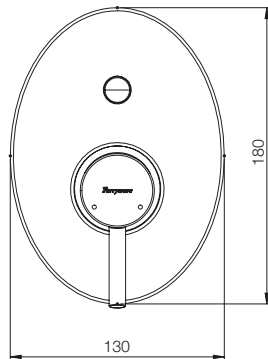
ULTRA HIGH FLOW DIVERTER UPPER TRIM G3385A1
