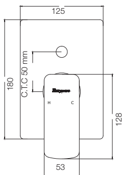
HIGH FLOW DIVERTER UPPER TRIM T2385A1 HIGH FLOW DIVERTER BODY G4887A1
