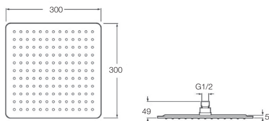
SS RAIN SHOWER WITHOUT ARM - SQUARE (300MM) T9992A1
