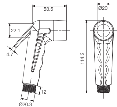
SPLASH WITH HOSE + HOOK T9805A1
