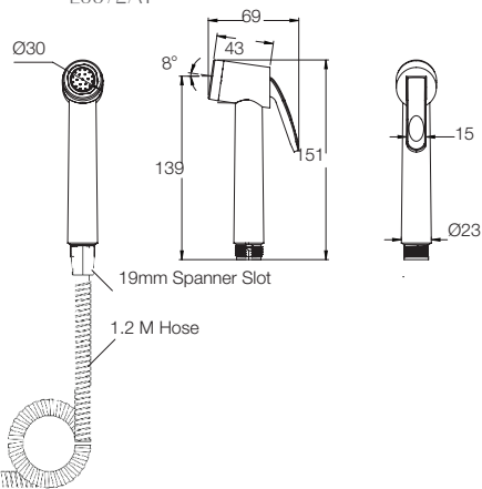
OVALO ANTI MICROBIAL WITH HOSE + HOOK E8372A1
