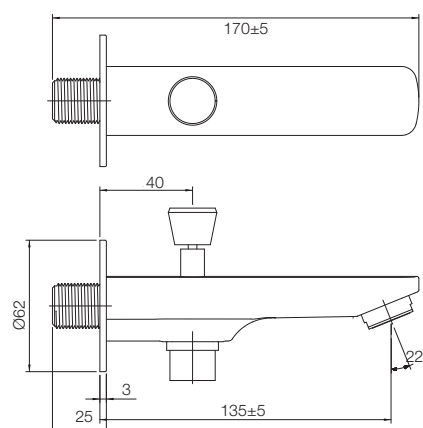
WALL SPOUT T1327A1
