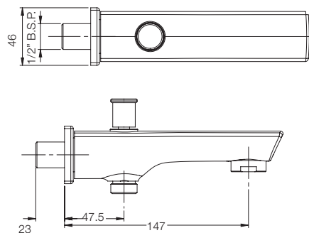
BATH SPOUT WITH DIVERTER G2328A1
