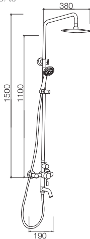
SHOWER COLUMN T4990A6
