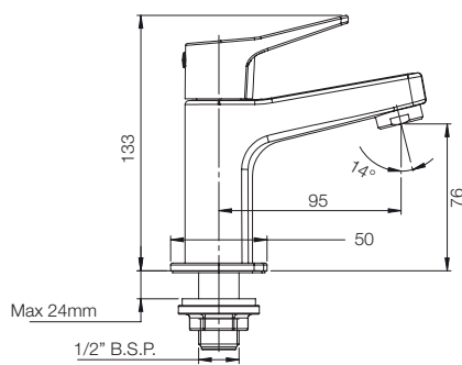
PILLAR TAP G5722A1
