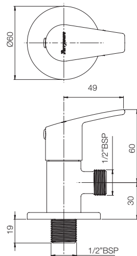
ANGLE VALVE G4807A1
