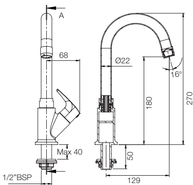
SWAN NECK PILLAR COCK WITH AERATOR G3203A1
