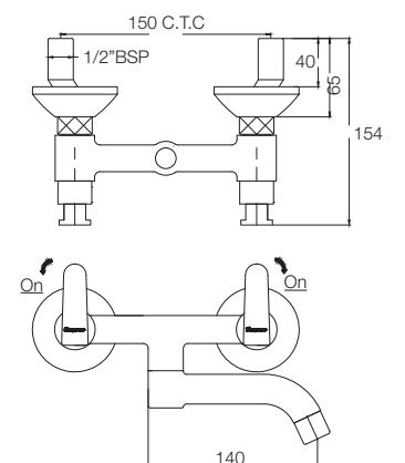
WALL MIXER NON TELEPHONIC T1941A1
