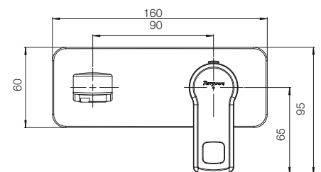
CONCEALED PILLAR COCK UPPER TRIM G3996A1 COMPATIBLE WITH CONCEALED PILLAR COCK BODY G2797A1
