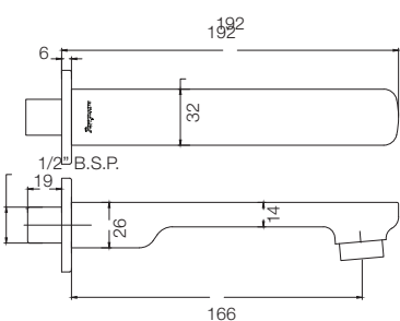
BATH SPOUT WITHOUT DIVERTER T2327A1
