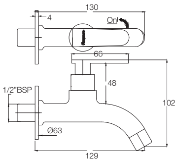
LONG BODY BIB COCK T1906A1
