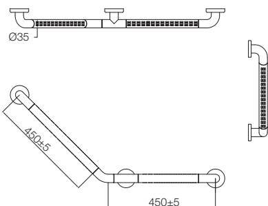
SLANTED SUPPORT BAR 135 DEGREE BEND (450MM) T6804A1 (White)
