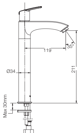
TALL PILLAR COCK G4864A1
