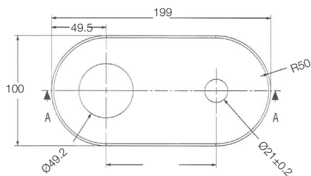
WALL MOUNTED BASIN MIXER T1356A1
