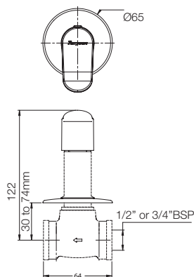
CSC-UPPER TRIM G2783A1 COMPATIBLE WITH CONCEALED BODY 1/2" & 3/4" G5052A1 G5053A1
