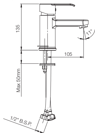
SINGLE LEVER BASIN MIXER G3815A1
