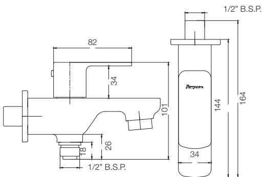
TWO WAY BIB COCK T2334A1
