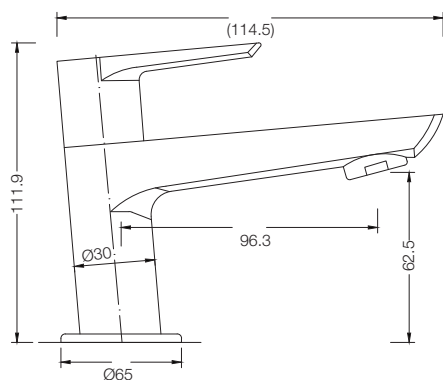
PILLAR COCK T4902A6
