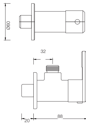
ANGLE VALVE G3907A1
