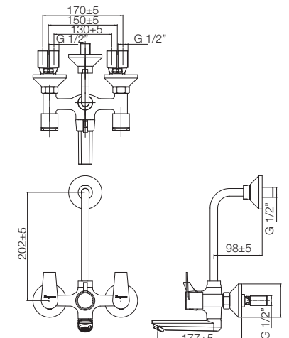
WALL MIXER 2-IN-1 T1354A1
