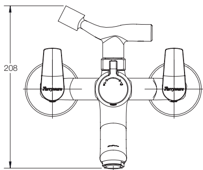
WALL MIXER WITH CRUTCH G3219A1
