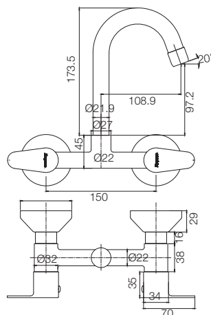
SINK MIXER T5035A1
