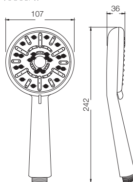
3 MODES, AIRMIX, HOSE + HOOK T9865A1
