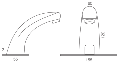
PILLAR COCK AC/DC T4701A1
