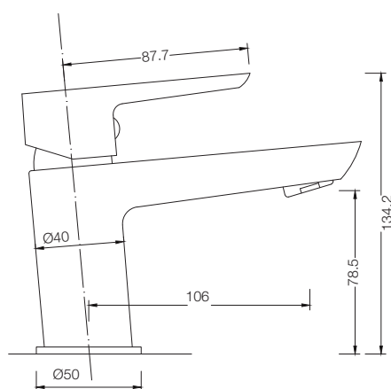
BASIN MIXER T4914A6
