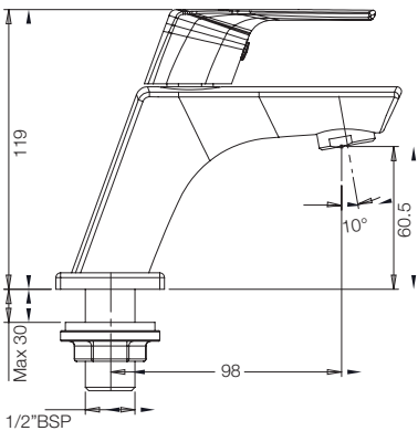
PILLAR COCK WITH AERATOR G2302A1
