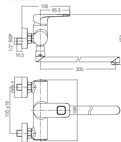
WALL MIXER WITH OHS G0654A1
