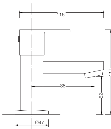
PILLAR COCK G5001A1 / T5001A1
