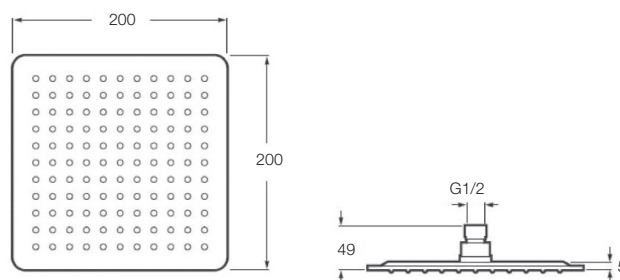
SS RAIN SHOWER WITHOUT ARM - SQUARE (200MM) T9975A1
