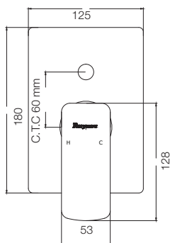
3 INLET DIVERTER UPPER TRIM T2384A1 COMPATIBLE WITH, 3-INLET CONCEALED DIVERTER BODY T9969A1
