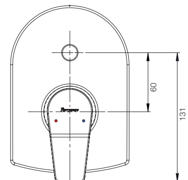
CONCEALED STOP COCK 1/2" & 3/4" G5711A1 COMPATIBLE WITH CONCEALED BODY 1/2" & 3/4" G5052A1 G5053A1
