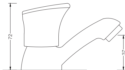
PILLAR COCK G4702A1
