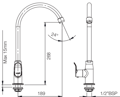
DECK MOUNTED SINK COCK G2738A1
