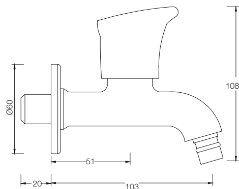
BIB COCK WITH NOZZLE G4769A1
