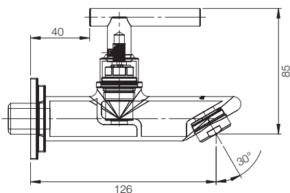
WALL SPOUT WITH DIVERTER G0628A1
