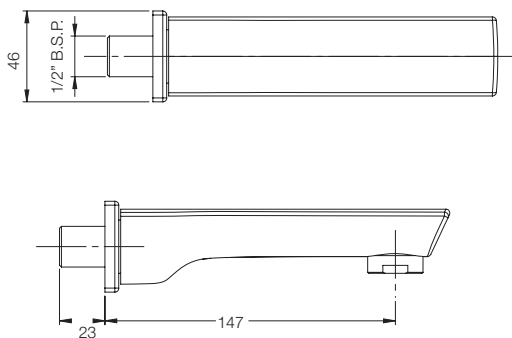
BATH SPOUT G2327A1
