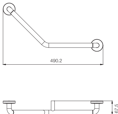
HAND GRIP 135° LEFT T6602A1
