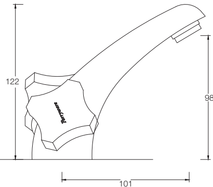
BASIN MIXER WITHOUT POP-UP G0214A1
