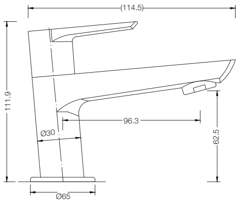
PILLAR COCK T4902A5
