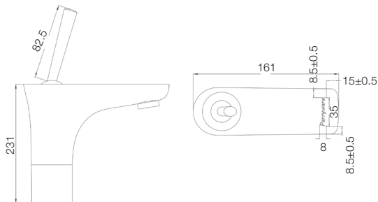
TALL BASIN MIXER T1810A1
