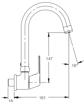
SINK COCK WITH SWINGING SPOUT G2321A1
