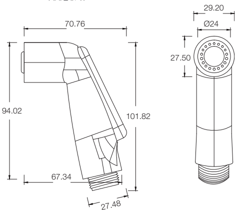
PRASEO WITH HOSE + HOOK T9920A1
