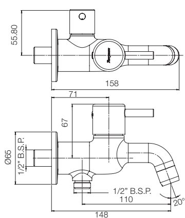
TWO WAY BIB COCK WITH AERATOR G3334A1
