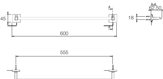
TOWEL RAIL (22") T6501A1
