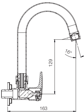
SINK COCK G3223A1
