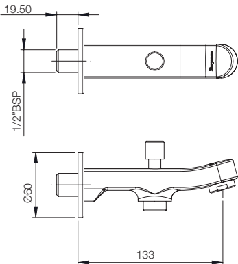
WALL SPOUT WITH DIVERTER G2728A1
