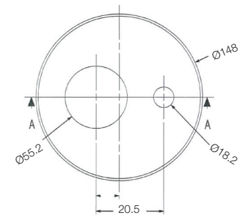
HIGH FLOW/ DIVERTER CUPPER TRIM T1385A1 HIGH FLOW/ DIVERTER BODY G4887A1
