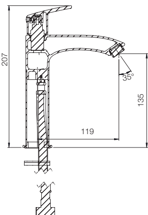
HIGH NECK PILLAR COCK (MEDIUM) G4868A1
