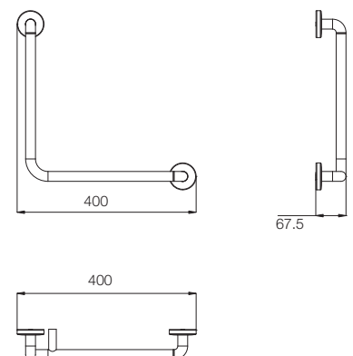
HAND GRIP 90° LEFT T6606A1
