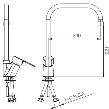
DECK MOUNTED SINGLE LEVER SINK MIXER G3145A1
