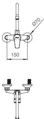
SINGLE LEVER SINK MIXER TOP OUTLET G321XA1
