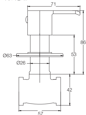
CONCEALED STOP COCK-3/4" WITH BODY T0712A1
