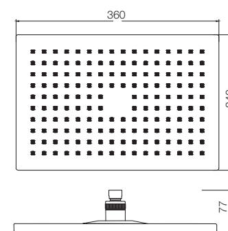
RAIN SHOWER WITHOUT ARM-ABS (360X240MM) T9979A1
