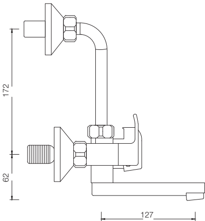
WALL MIXER 2-IN-1 WITH FLAT FLANGE G3816A1
