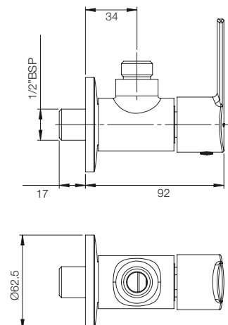
ANGLE VALVE G3107A1
