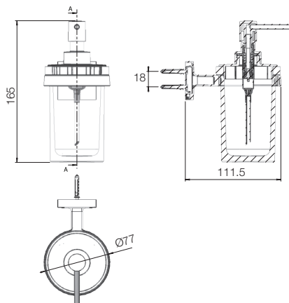
SOAP DISPENSER T6513A1
