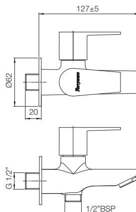
TWO WAY BIB COCK T1381A1
