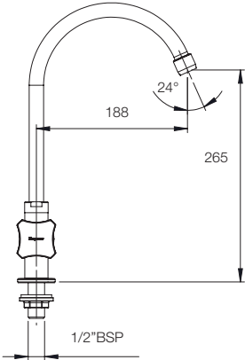
DECK MOUNTED SINK COCK G0238A1
