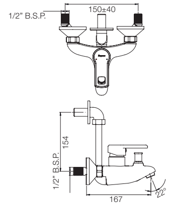
SINGLE LEVER WALL MIXER WITH BEND G3954A1
