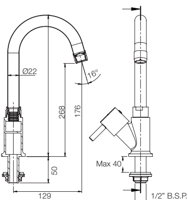
SWAN NECK PILLAR COCK G3303A1
