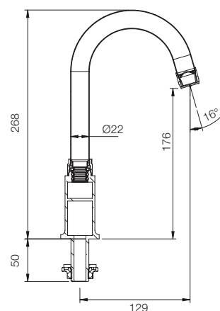
SWAN NECK PILLAR COCK G4803A1
