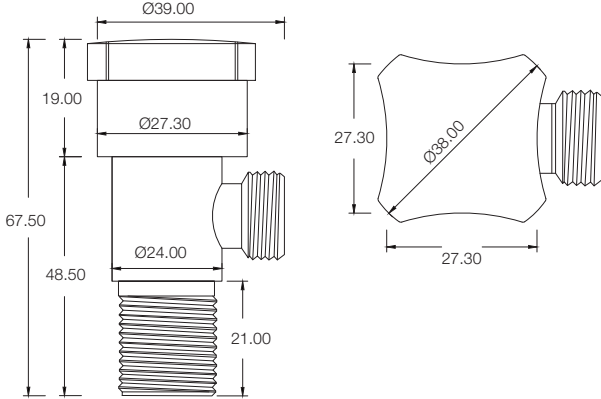
ANGLE VALVE G0253A1
