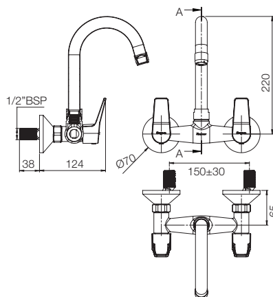
WALL MOUNTED SINK MIXER (2 KNOBS) G5735A1
