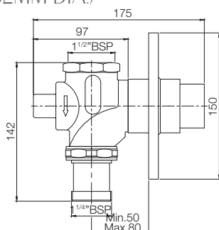
CONCEALED FLUSH VALVE (40MM DIA.) CONCEALED FLUSH VALVE (32MM DIA.)
