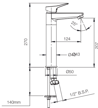
TALL BASIN MIXER G5746A1
