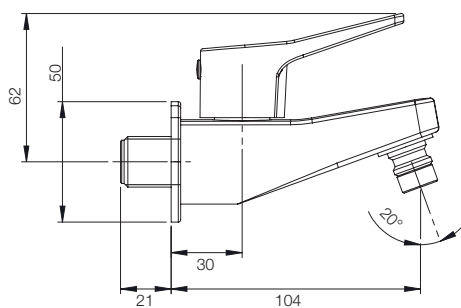
BIB COCK WITH NOZZLE G5779A1
