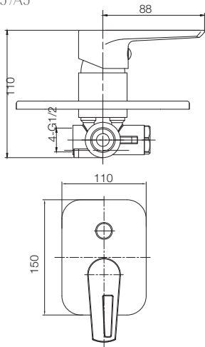
CONCEALED SHOWER MIXER T4957A5
