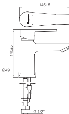
SINGLE LEVER BASIN MIXER T132DA1
