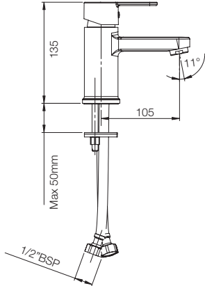
BASIN MIXER (COLD START) G5265A1
