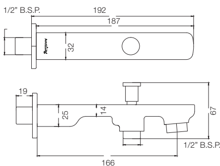
BATH SPOUT WITH DIVERTER T2328A1
