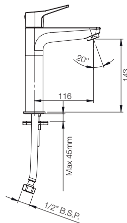
MEZZO PILLAR TAP G572BA1
