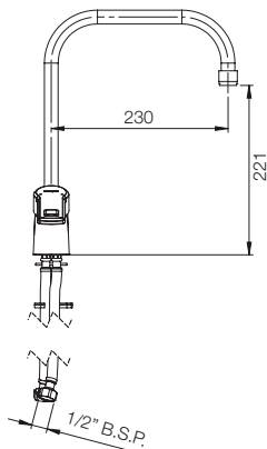
DECK MOUNTED S/L SINK MIXER G3937A1
