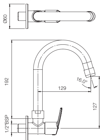
WALL MOUNTED SINK COCK G4836A1
