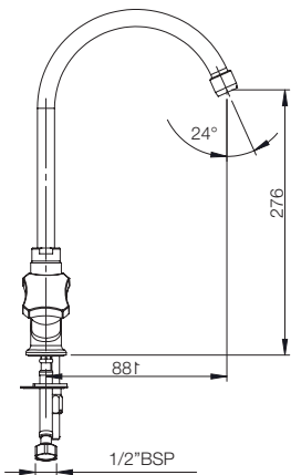
DECK MOUNTED SINK MIXER TWO KNOB G0245A1
