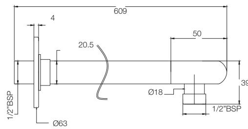
LONG SHOWER ARM 24" T9949A1
