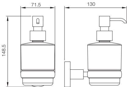
SOAP DISPENSER T4988A5
