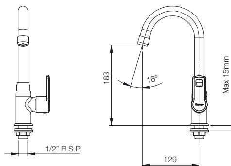
SWAN NECK PILLAR COCK G3903A1
