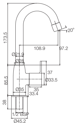
SWAN NECK PILLAR COCK T4668A1
