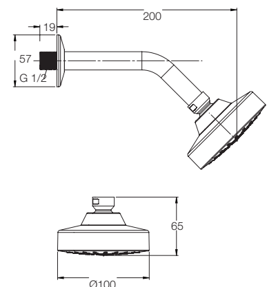
PLUTO OVERHEAD SHOWER ARM (100MM) E8380A1
