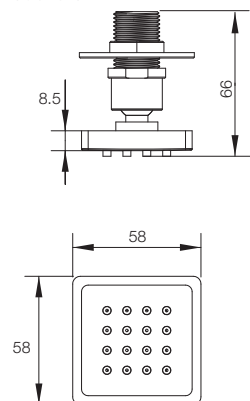
SOMA - SQUARE BODY JET T9878A1
