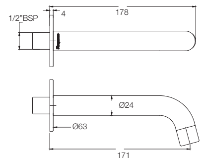
BATH SPOUT WITHOUT DIVERTER T1927A1
