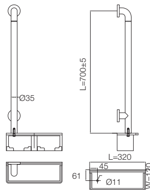
L SHAPE SUPPORT BAR WITH SHELF (700MM) T6808A1 (White)
