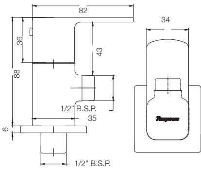
ANGLE VALVE T2307A1
