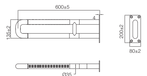
U SHAPED - LIFT SUPPORT BAR NON-FOLDING T6807A1 (White)
