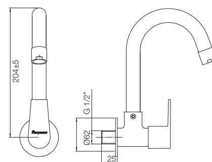
SINK COCK WALL MOUNTED T1321A1
