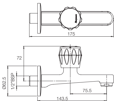
BIB COCK WITH AERATOR G1469A1
