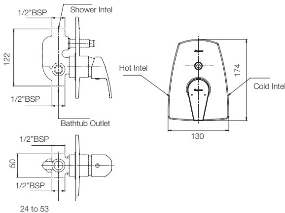
CONCEALED DIVERTER UPPER TRIM G4850A1 COMPATIBLE WITH CONCEALED DIVERTER BODY G5051A1
