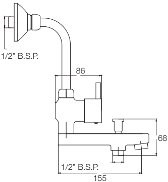
WALL MIXER 3-IN-1 T0717A1
