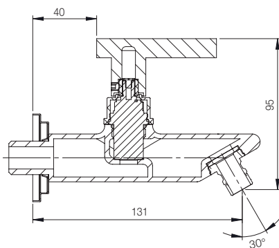
BIB COCK WITH NOZZLE G3379A1
