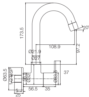
WALL MOUNTED SINK COCK T4621A1
