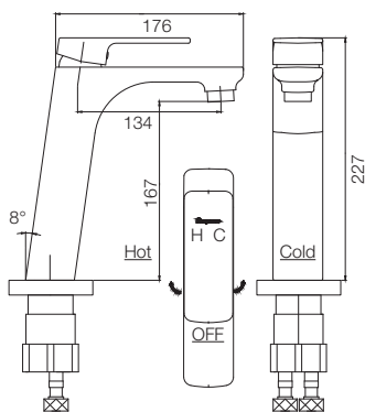
SINGLE LEVER BASIN MIXER 9" T2346A1
