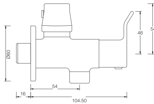
TWO-WAY ANGLE VALVE G271YA1
