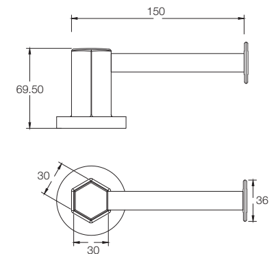
PAPER HOLDER T6005A1
