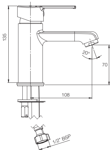
BASIN MIXER N G3165A1
