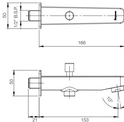
WALL SPOUT WITH DIVERTER G5728A1
