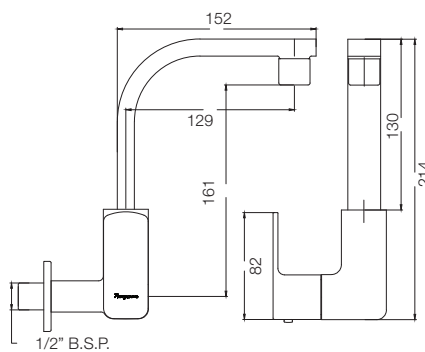
SINK COCK T2321A1
