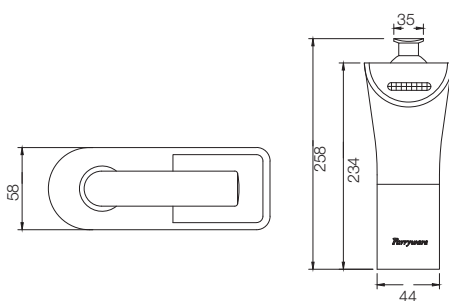
TALL BASIN MIXER T171MA1
