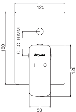
CONCEALED DIVERTER UPPER TRIM T2350A1 COMPATIBLE WITH CONCEALED DIVERTER BODY G5051A1
