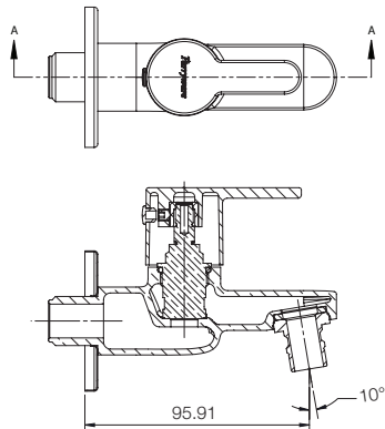
BIB COCK WITH NOZZLE G5279A1
