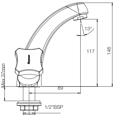
SWAN NECK PILLAR COCK G0268A1
