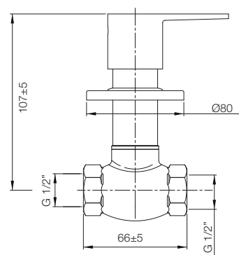
CSC 15 MM WITH WALL FLANGE 1/2" WITH BODY T1311A1
