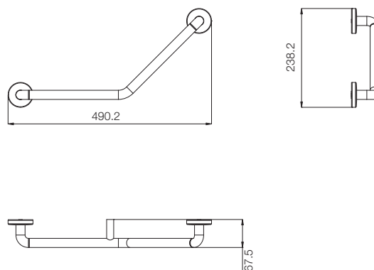
HAND GRIP 135° RIGHT T6603A1
