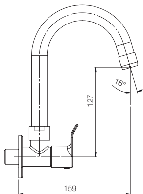
WALL MOUNTED SINK COCK G2721A1
