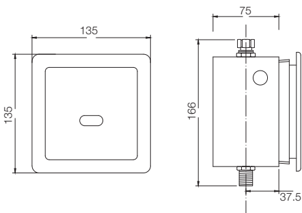
FLUSH VALVE AC/DC T471BA1
