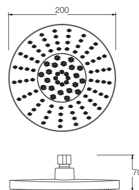
WATER SAVING GREY FACEPLATE SHOWER (200MM) T9844A1
