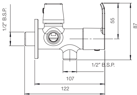
TWO WAY ANGLE VALVE G3843A1
