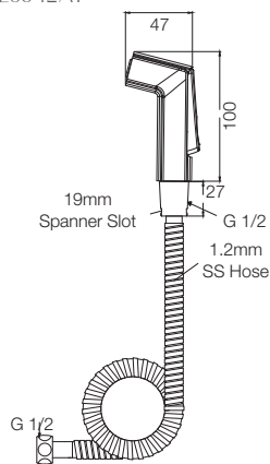
CRUST WITH SS HOSE+ HOOK E8342A1
