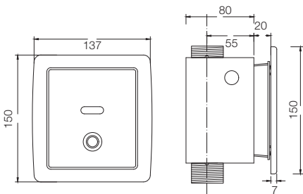
FLUSH VALVE WC AC/ DC WITH BUTTON T471EA1
