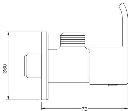
ANGLE VALVE G3807A1
