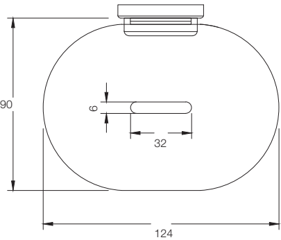
SOAP DISH T6902A1
