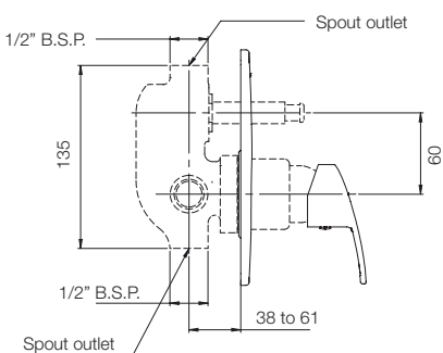
HIGH FLOW DIVERTER UPPER TRIM G4885A1 HIGH FLOW DIVERTER BODY G4887A1
