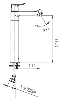
TALL PILLAR COCK WITH AERATOR G2742A1
