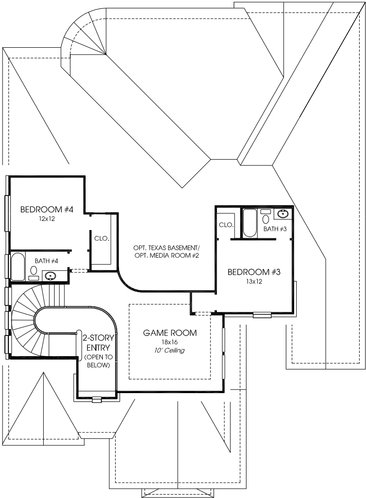
SECOND FLOOR
