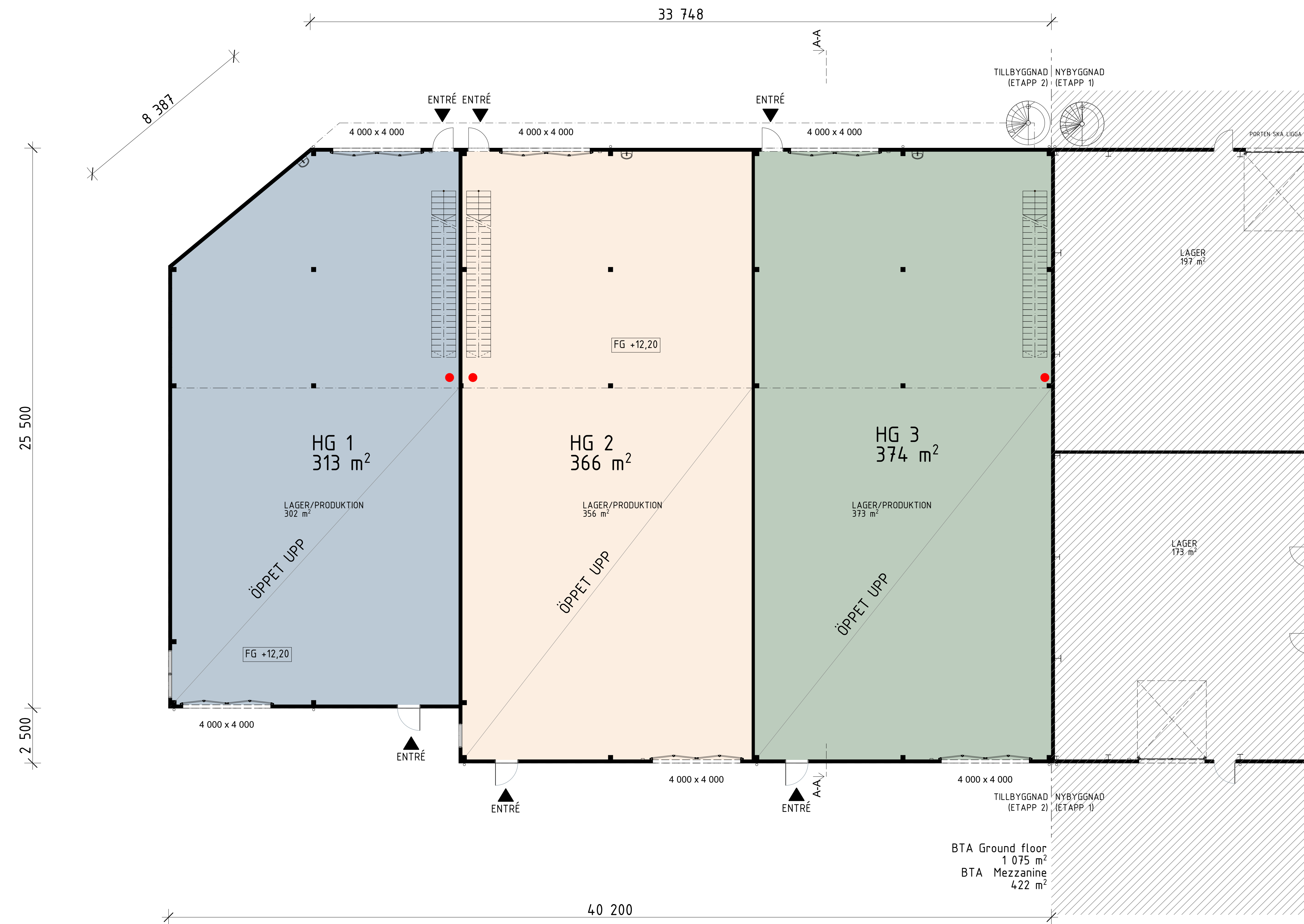
PLAN 1 Ground floor 1:100
