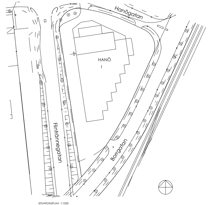
SITUATIONSPLAN 1:1000
