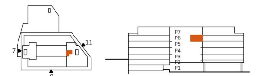
Situationsplan
