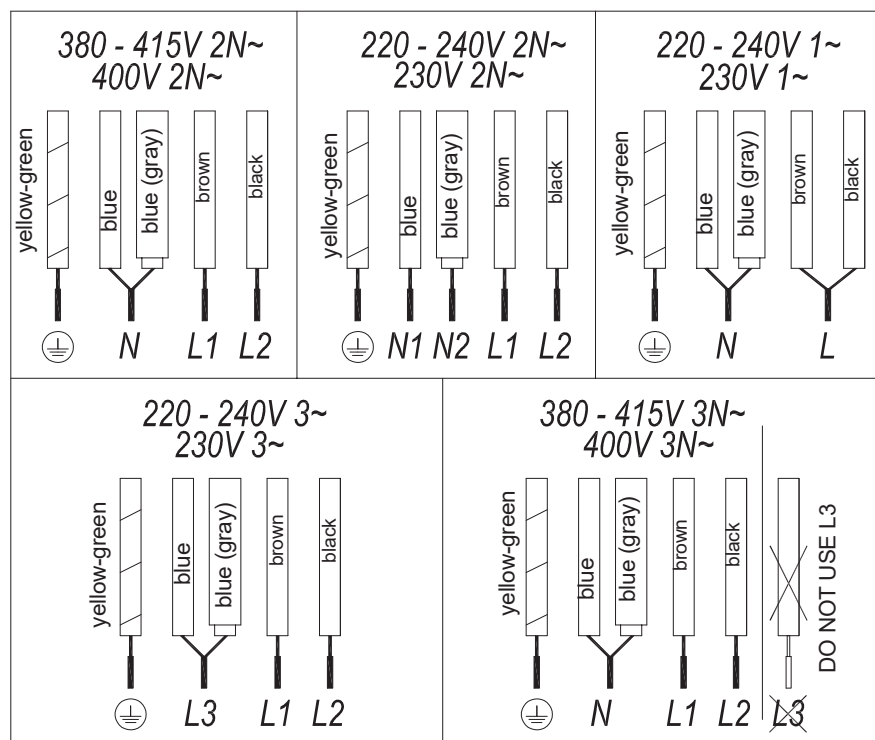
Fig.2a (5 WIRES)
