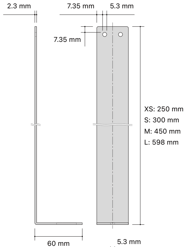
Mount Parts - Arm Plate XS / S / M / L
