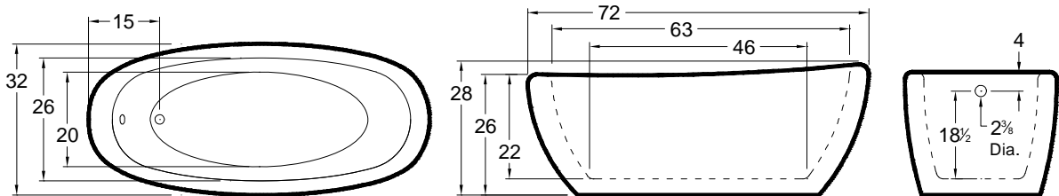
All bathtub dimensions are \pm 1/2 ".
