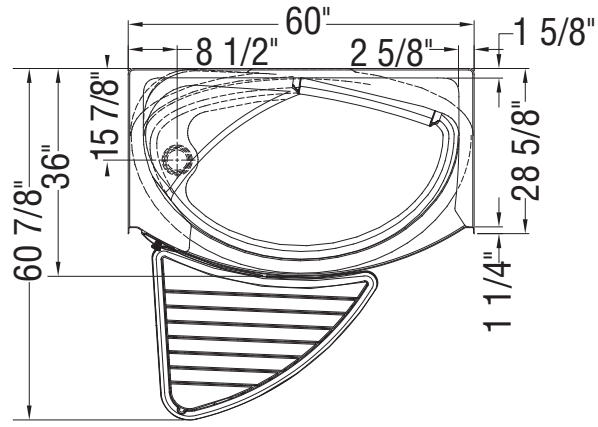
Left-hand seat with optional dry platform
