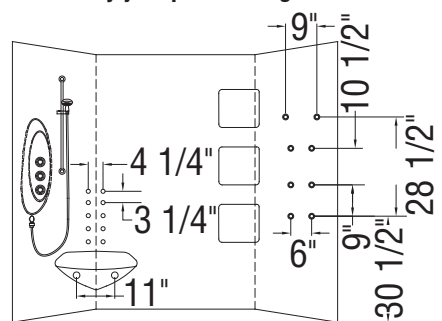
MAAX IES 3/4 with Body jets positioning
