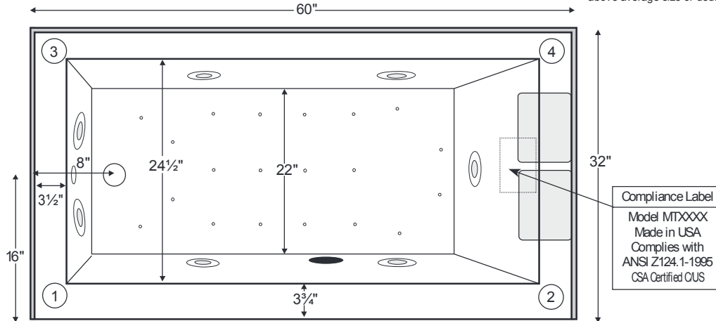
Numbered areas on tub deck represent possible locations to install cleaning systems, faucets and other fixtures.
