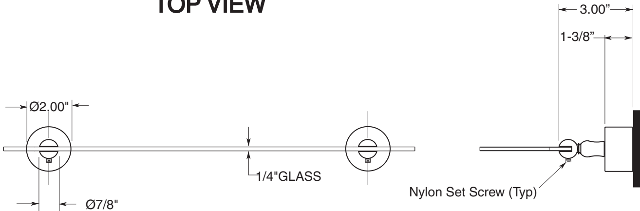
TOP VIEW
