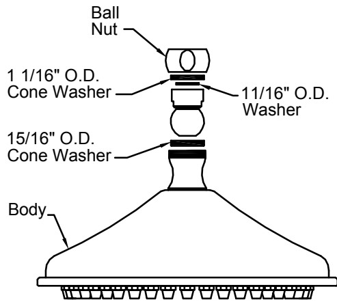
Exploded View
