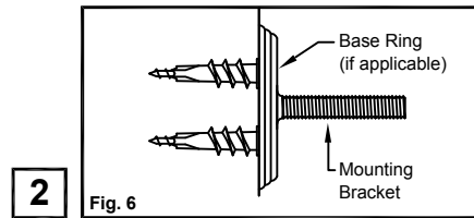
Towel Ring
