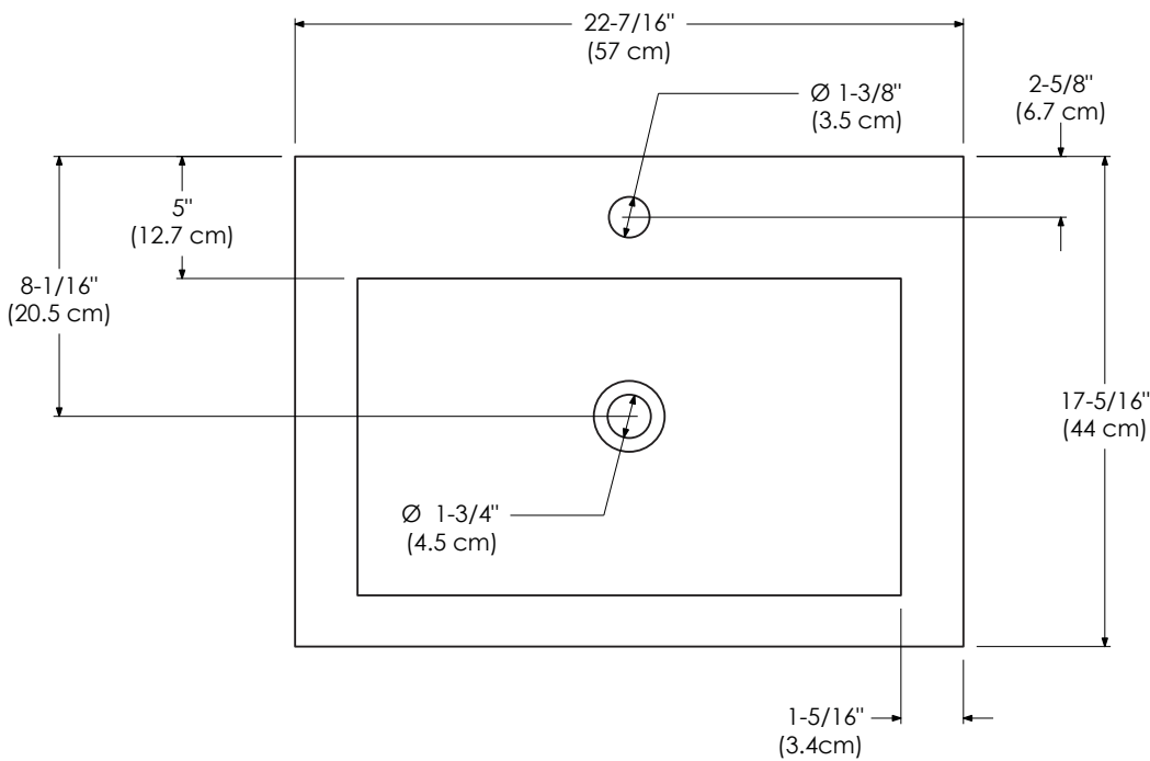
TOP VIEW
