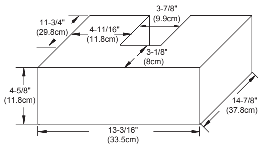
BOTTOM DRAWER Exterior Dimensions
