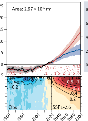
g Mediterranean Sea OHC
