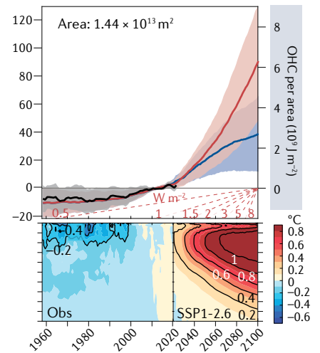
h Arctic Ocean OHC (65° N to 90° N)
