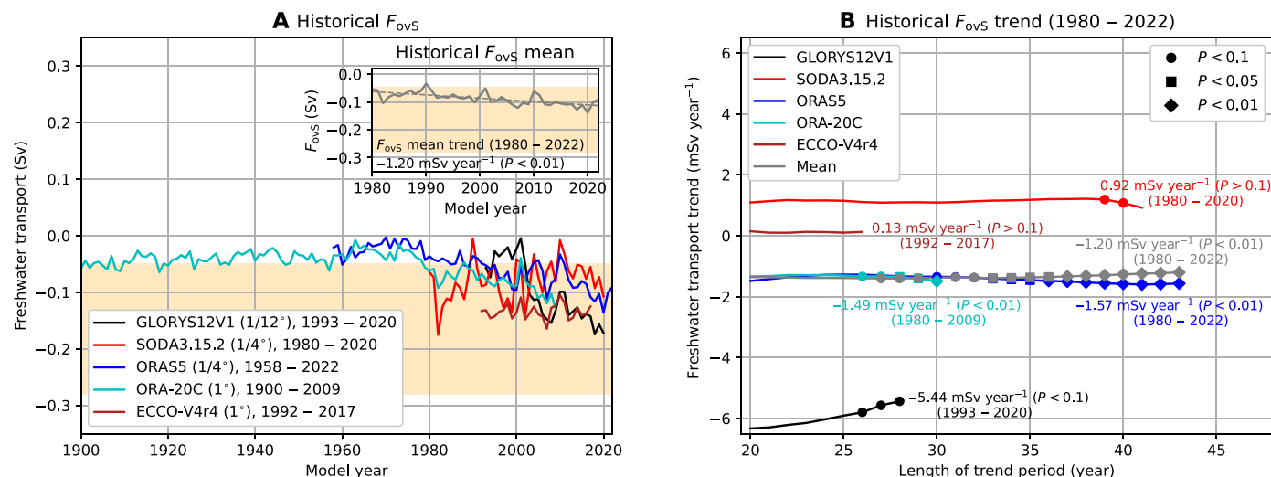
Fig. 6. Historical F_{ovs} and trend. (A) Historical F_{ovs} for five different reanalysis and assimilation products. The horizontal resolution for the ocean component and the time span is indicated in the legend. The F_{ovs} multi-reanalysis mean (inset) is the yearly average over all available products. The yellow shading indicates observed ranges for F_{ovs} . (B) Present-day (1980 to 2022) F_{ovs} trend. We use a sliding window (varying length of 20 to 43 years) over the available time series (1980 to 2022) to determine all F_{ovs} trends and then determine the mean trend, which is displayed for each reanalysis product and the multi-reanalysis mean. The markers indicate the least significant [two-sided t test (23)] trend for a given sliding window, and the trends at the maximum sliding window length (only one trend possible) are also displayed.
