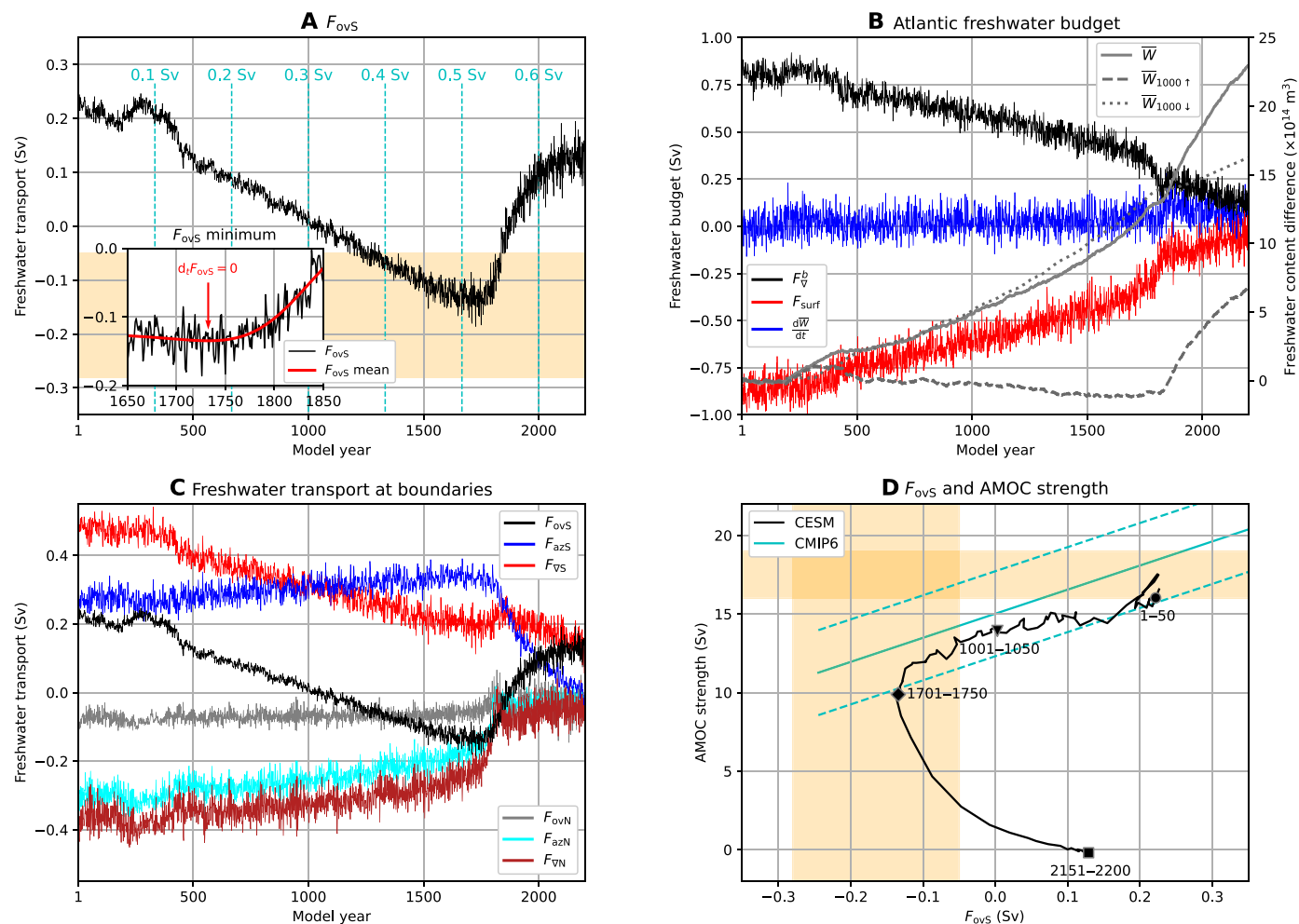
Fig. 4. Freshwater transport by the AMOC and Atlantic Ocean freshwater budget. (A) Freshwater transport by the AMOC at 34^{\circ}\text{S} , F_{\text{ovS}} . The cyan-colored lines indicate the magnitude of F_{\text{H}} . Inset: Zoom in around F_{\text{ovS}} minimum (model year 1732; fig. S1, C and D), where the F_{\text{ovS}} mean is determined from cubic splines (here for 50-year averages, see Materials and Methods). (B) Atlantic Ocean freshwater content ( \bar{W} ) difference (with respect to time mean over model years 1 to 50) and with the freshwater content difference of the upper 1000 m ( \bar{W}_{1000\uparrow} ) and below 1000 m ( \bar{W}_{1000\downarrow} ). The freshwater budget components of the freshwater convergence ( F_{\text{V}}^{\text{b}} , freshwater transport at 34^{\circ}\text{S} , 60^{\circ}\text{N} , and the Strait of Gibraltar), surface freshwater fluxes ( F_{\text{surf}} ), and changes in the freshwater content ( \frac{d\bar{W}}{dt} ). (C) Meridional freshwater transport at the Atlantic boundaries of 34^{\circ}\text{S} and 60^{\circ}\text{N} for the overturning component ( F_{\text{ovS}} and F_{\text{ovN}} ), the azonal (gyre) component ( F_{\text{azS}} and F_{\text{azN}} ), and the total freshwater transport ( F_{\text{vS}} and F_{\text{vN}} ). Positive (negative) values indicate the northward transport of net fresh water (salinity). (D) F_{\text{ovS}} and AMOC strength over time. The time series are displayed as 25-year averages (to reduce the variability of the time series). The markers indicate the 50-year average over a particular period. The cyan-colored curve indicates the present-day (1994 to 2020) CMIP6 regression and 1 SD (37). The yellow shading in (A) and (D) indicates observed ranges (21, 42, 60, 61) for F_{\text{ovS}} and AMOC strength.
