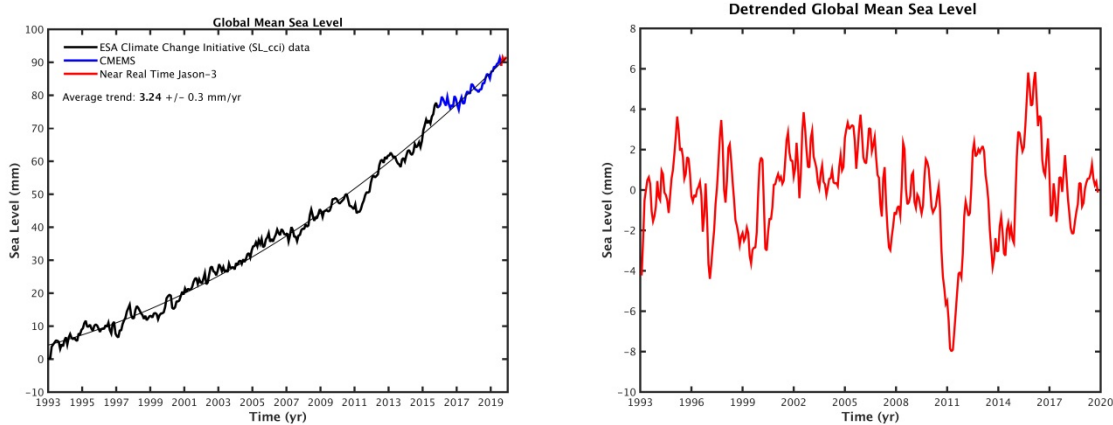
Figure 6: Global mean sea level evolution for January 1993–October 2019 from high-precision altimetry. The thin black curve is a quadratic function that best fits the data. (right) Detrended global mean sea level over the same period (the difference between the smooth quadratic function and the measured values in the left panel).
