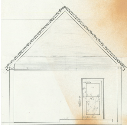
SECTION 1:20
