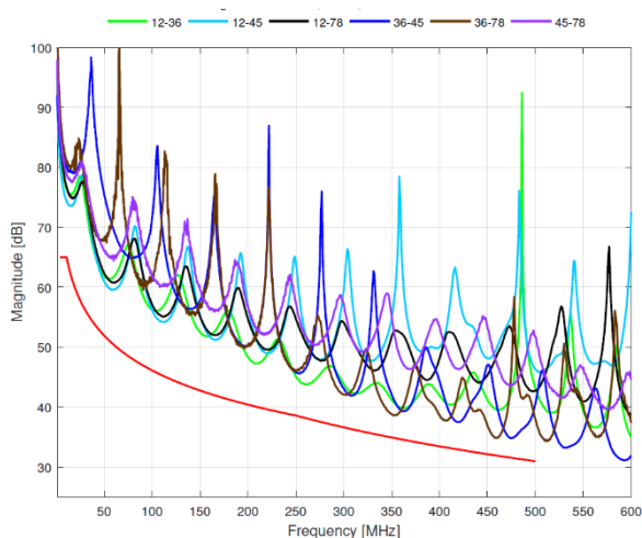
Typical NEXT Cat. 6A CL /s patch cord 2m
