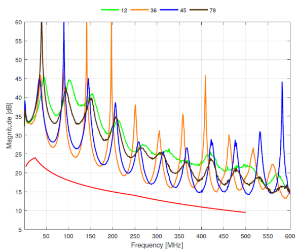
Typical Return Loss Cat.6A CL /u patch cord 2m
