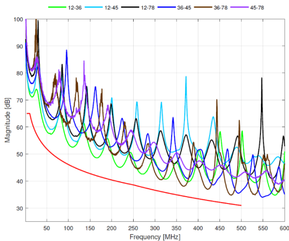
Typical NEXT Cat. 6A CL /u patch cord 2m
