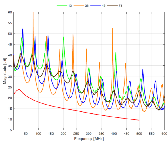
Typical Return Loss Cat. 6A CL /s patch cord 2m
