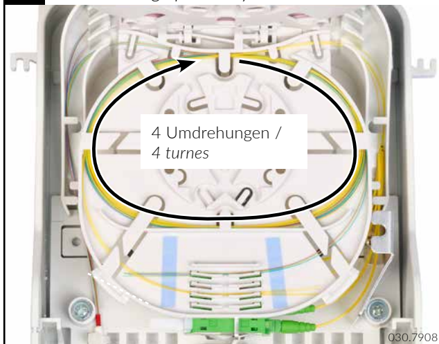
F3 Faserführung Spleisskassette / Fiber routing splice tray
